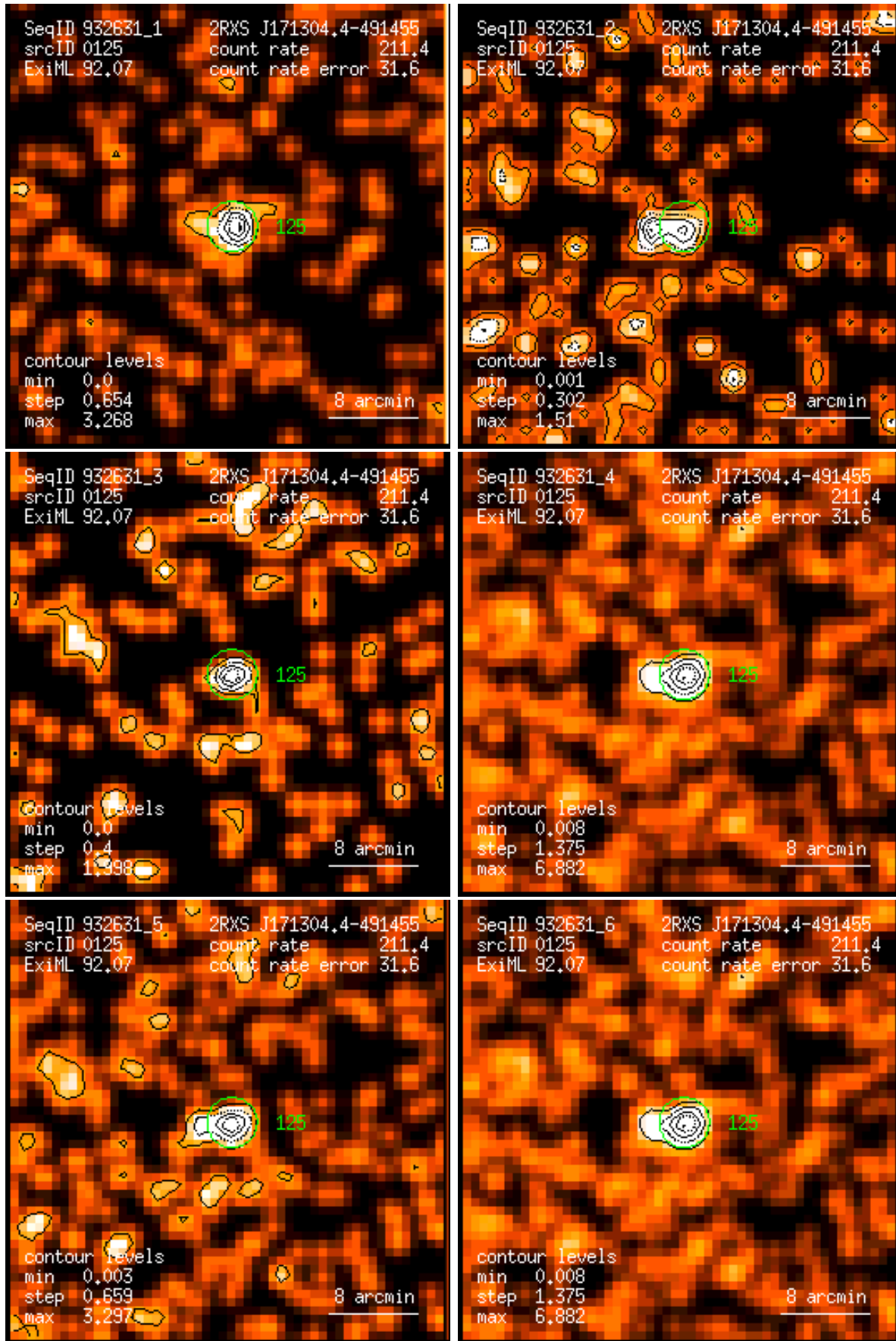
Figure 125: RASS 932631: detection 0125: band rate images, Gaussian filter: (1) PSPC channels 11 – 41, (2) 52 – 90, (3) 91 – 201, (4) 11 – 235, (5) 52 – 201, (6) 11 – 201. Broad band rates in counts/ks. Band rate contour levels in counts/ks/arcmin 2 .
