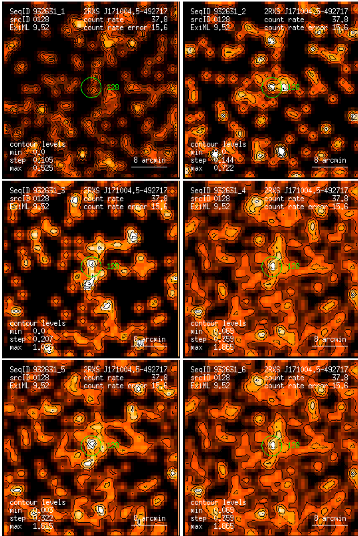
Figure 128: RASS 932631: detection 0128: band rate images, Gaussian filter: (1) PSPC channels 11 – 41, (2) 52 – 90, (3) 91 – 201, (4) 11 – 235, (5) 52 – 201, (6) 11 – 201. Broad band rates in counts/ks. Band rate contour levels in counts/ks/arcmin 2 .
