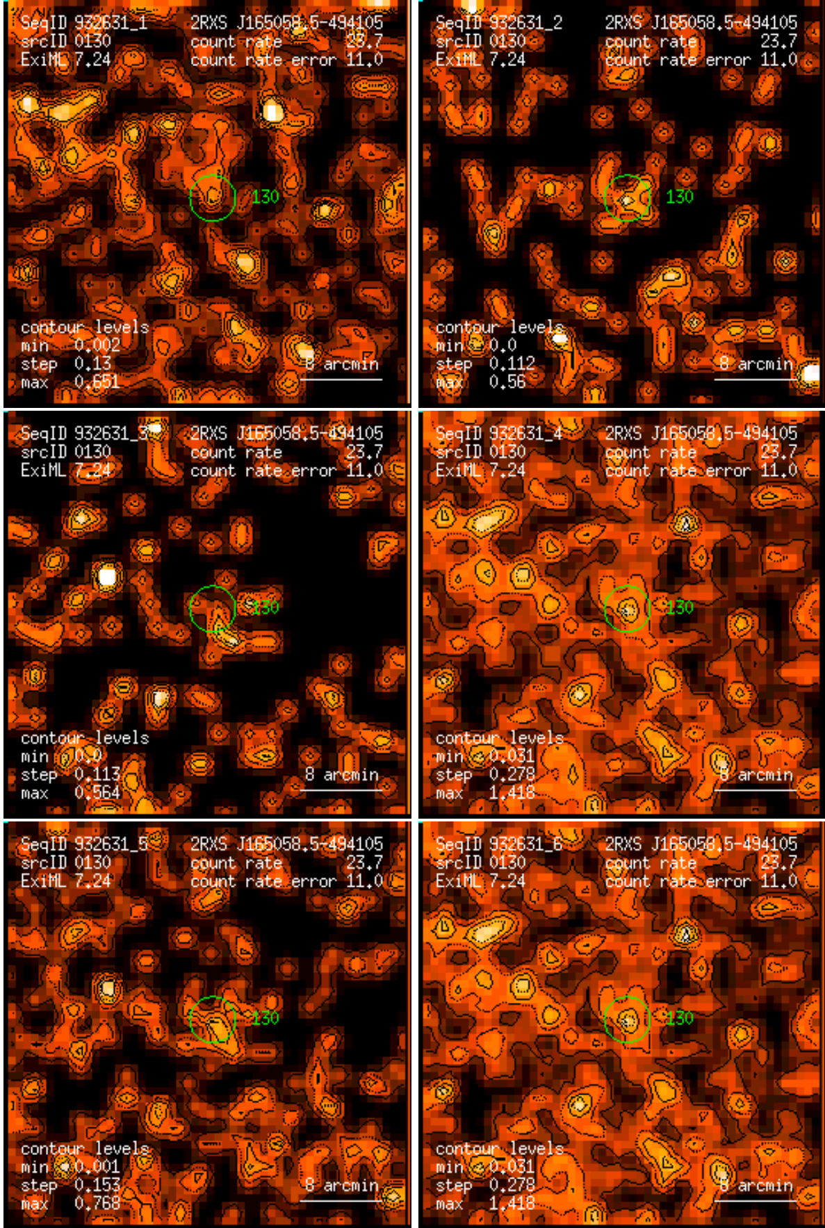
Figure 130: RASS 932631: detection 0130: band rate images, Gaussian filter: (1) PSPC channels 11 – 41, (2) 52 – 90, (3) 91 – 201, (4) 11 – 235, (5) 52 – 201, (6) 11 – 201. Broad band rates in counts/ks. Band rate contour levels in counts/ks/arcmin 2 .
