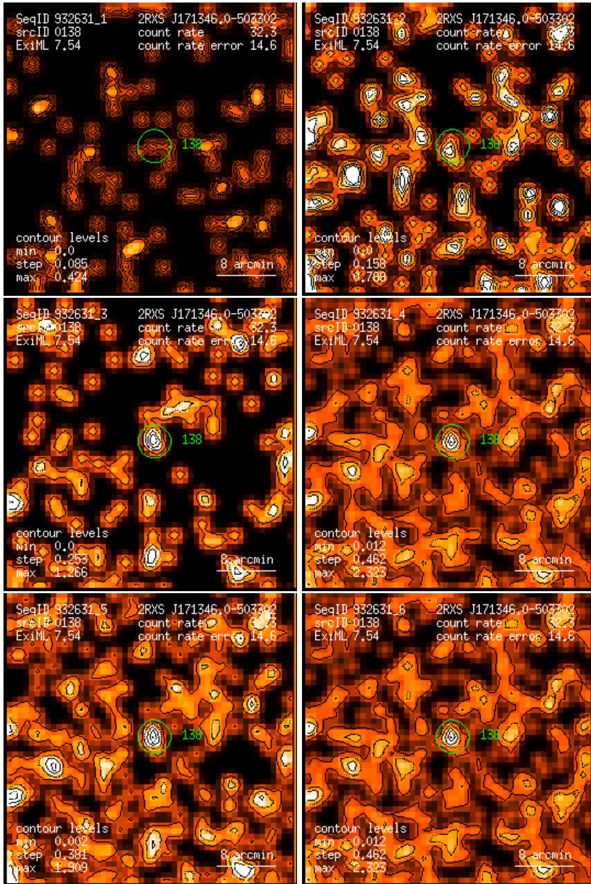
Figure 138: RASS 932631: detection 0138: band rate images, Gaussian filter: (1) PSPC channels 11 – 41, (2) 52 – 90, (3) 91 – 201, (4) 11 – 235, (5) 52 – 201, (6) 11 – 201. Broad band rates in counts/ks. Band rate contour levels in counts/ks/arcmin 2 .
