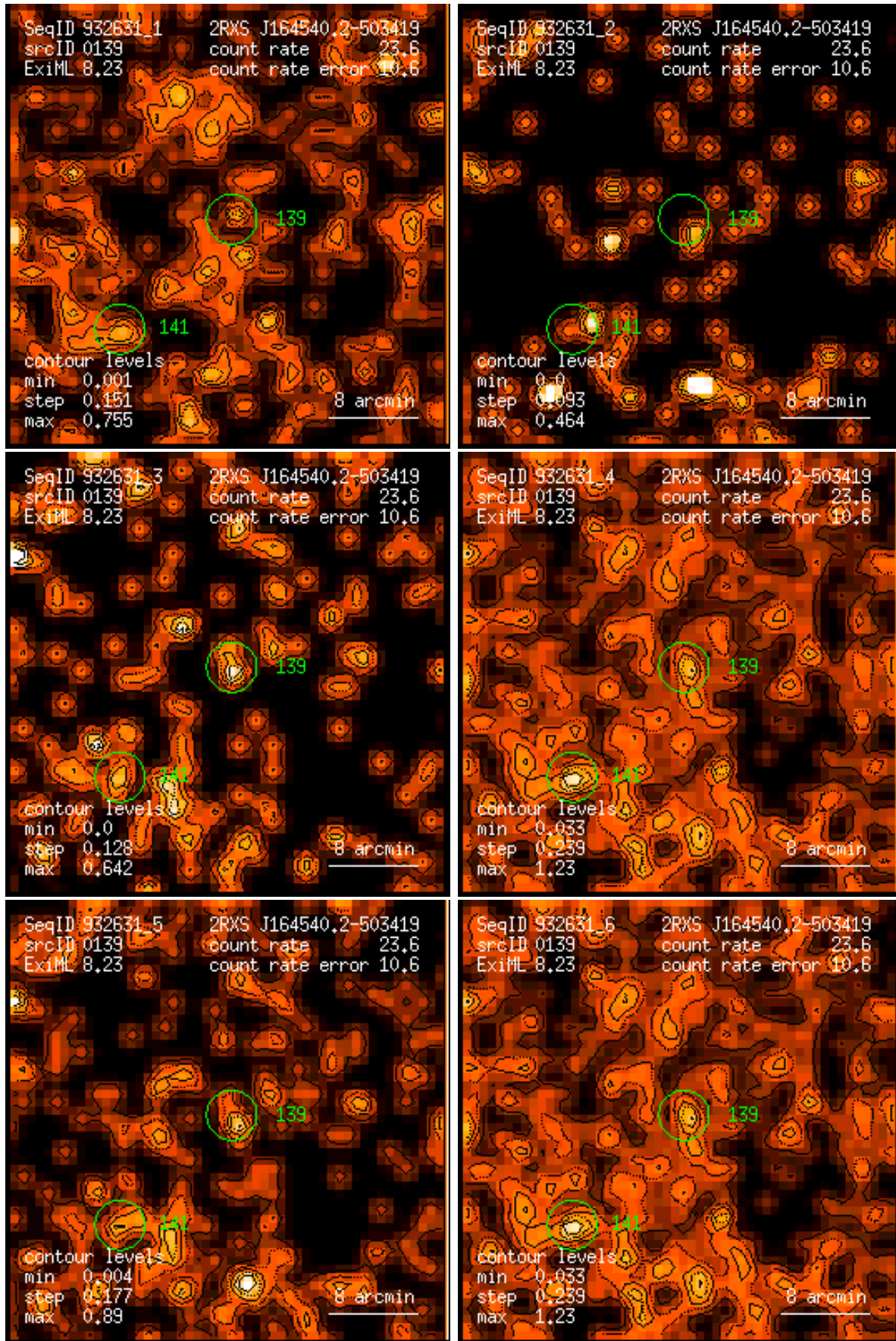
Figure 139: RASS 932631: detection 0139: band rate images, Gaussian filter: (1) PSPC channels 11 – 41, (2) 52 – 90, (3) 91 – 201, (4) 11 – 235, (5) 52 – 201, (6) 11 – 201. Broad band rates in counts/ks. Band rate contour levels in counts/ks/arcmin 2 .
