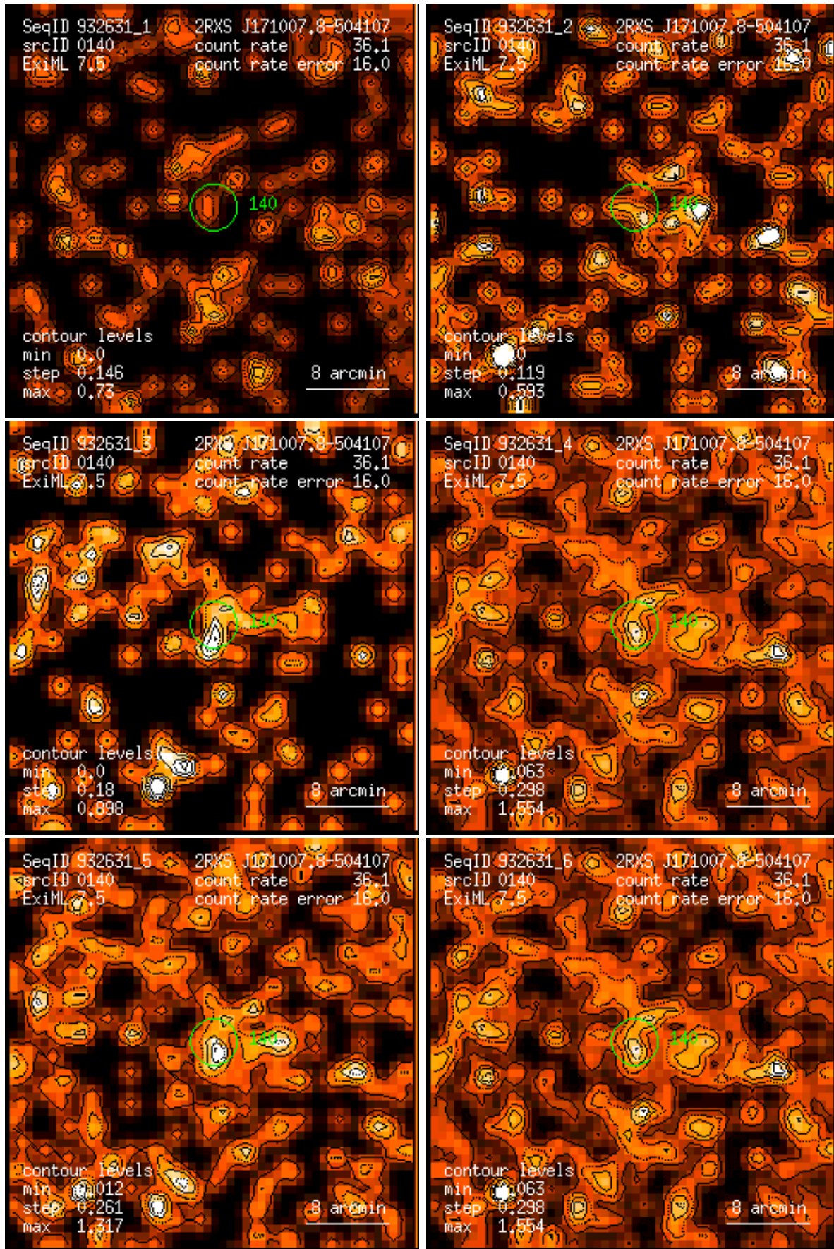
Figure 140: RASS 932631: detection 0140: band rate images, Gaussian filter: (1) PSPC channels 11 – 41, (2) 52 – 90, (3) 91 – 201, (4) 11 – 235, (5) 52 – 201, (6) 11 – 201. Broad band rates in counts/ks. Band rate contour levels in counts/ks/arcmin 2 .
