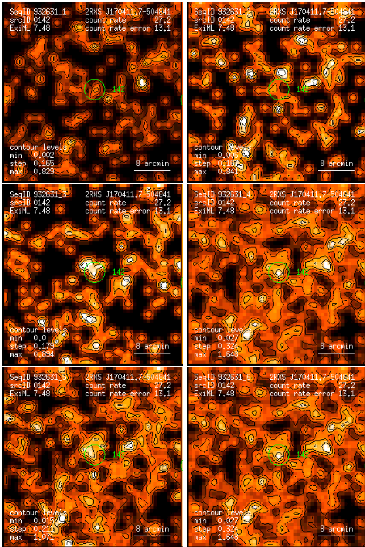
Figure 142: RASS 932631: detection 0142: band rate images, Gaussian filter: (1) PSPC channels 11 – 41, (2) 52 – 90, (3) 91 – 201, (4) 11 – 235, (5) 52 – 201, (6) 11 – 201. Broad band rates in counts/ks. Band rate contour levels in counts/ks/arcmin 2 .
