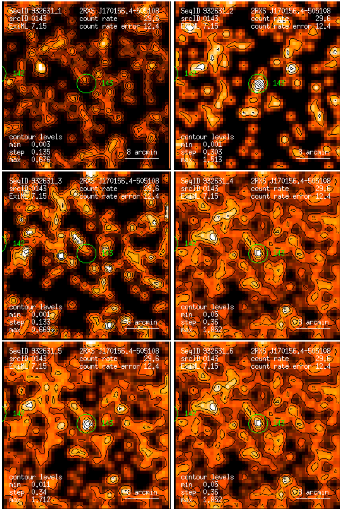
Figure 143: RASS 932631: detection 0143: band rate images, Gaussian filter: (1) PSPC channels 11 – 41, (2) 52 – 90, (3) 91 – 201, (4) 11 – 235, (5) 52 – 201, (6) 11 – 201. Broad band rates in counts/ks. Band rate contour levels in counts/ks/arcmin 2 .
