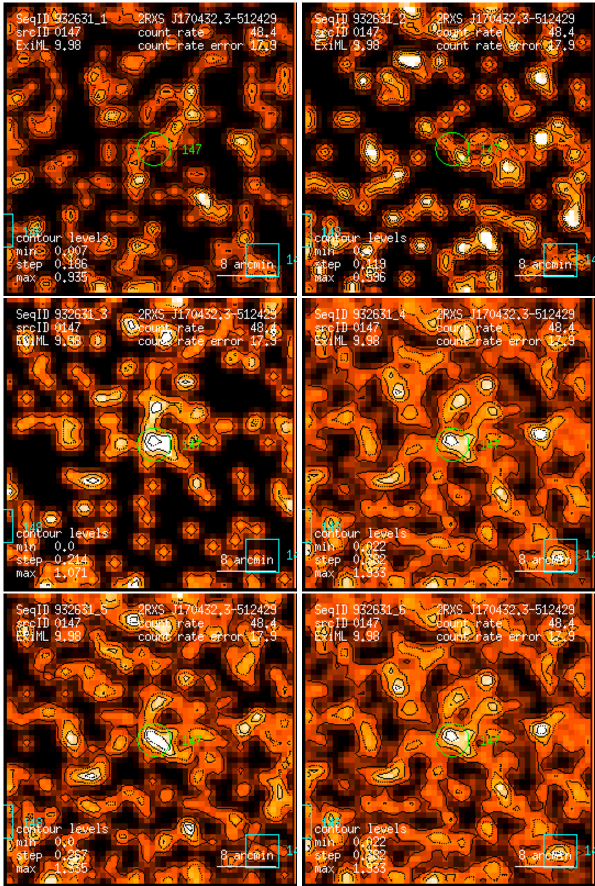
Figure 147: RASS 932631: detection 0147: band rate images, Gaussian filter: (1) PSPC channels 11 – 41, (2) 52 – 90, (3) 91 – 201, (4) 11 – 235, (5) 52 – 201, (6) 11 – 201. Broad band rates in counts/ks. Band rate contour levels in counts/ks/arcmin 2 .
