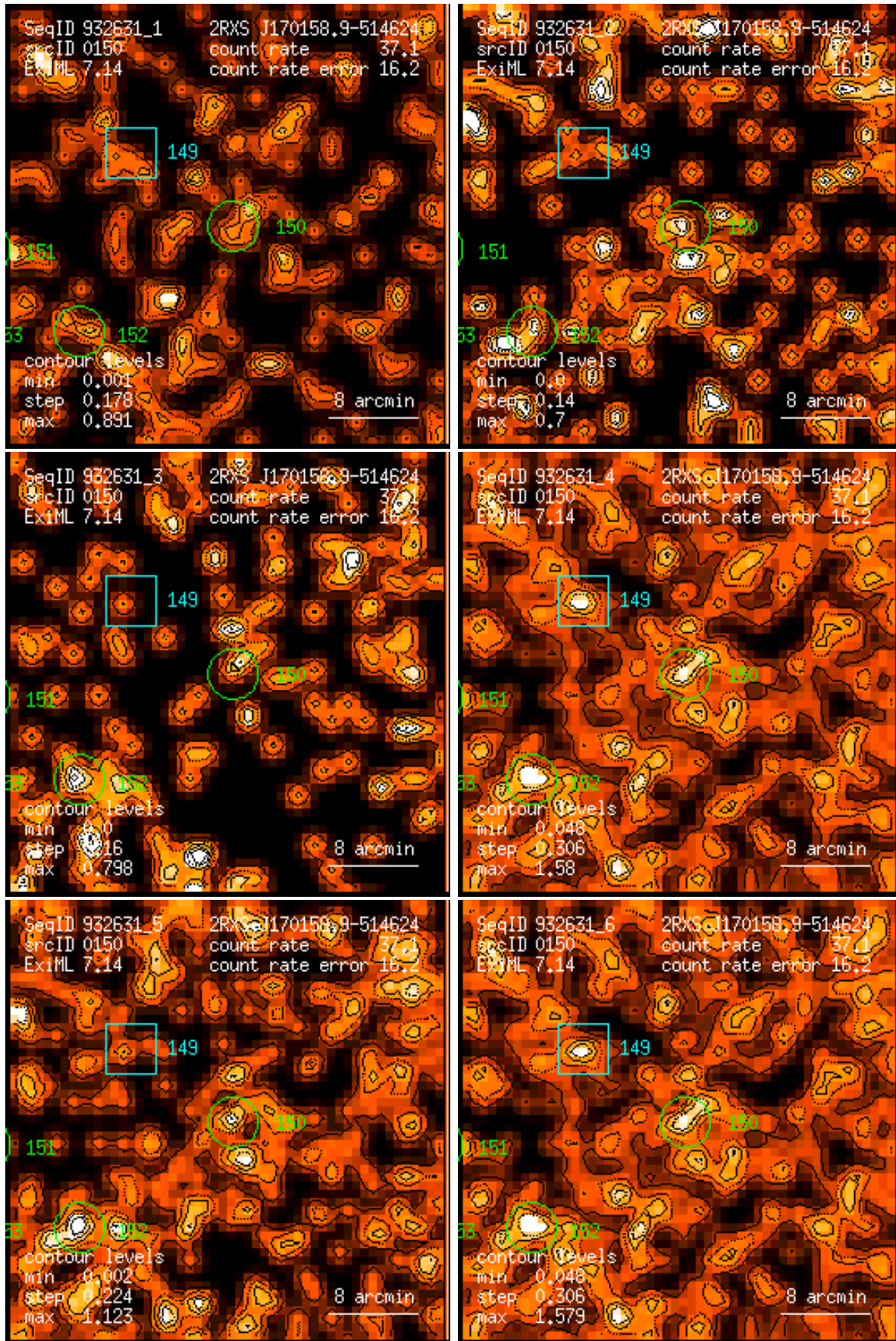
Figure 150: RASS 932631: detection 0150: band rate images, Gaussian filter: (1) PSPC channels 11 – 41, (2) 52 – 90, (3) 91 – 201, (4) 11 – 235, (5) 52 – 201, (6) 11 – 201. Broad band rates in counts/ks. Band rate contour levels in counts/ks/arcmin 2 .
