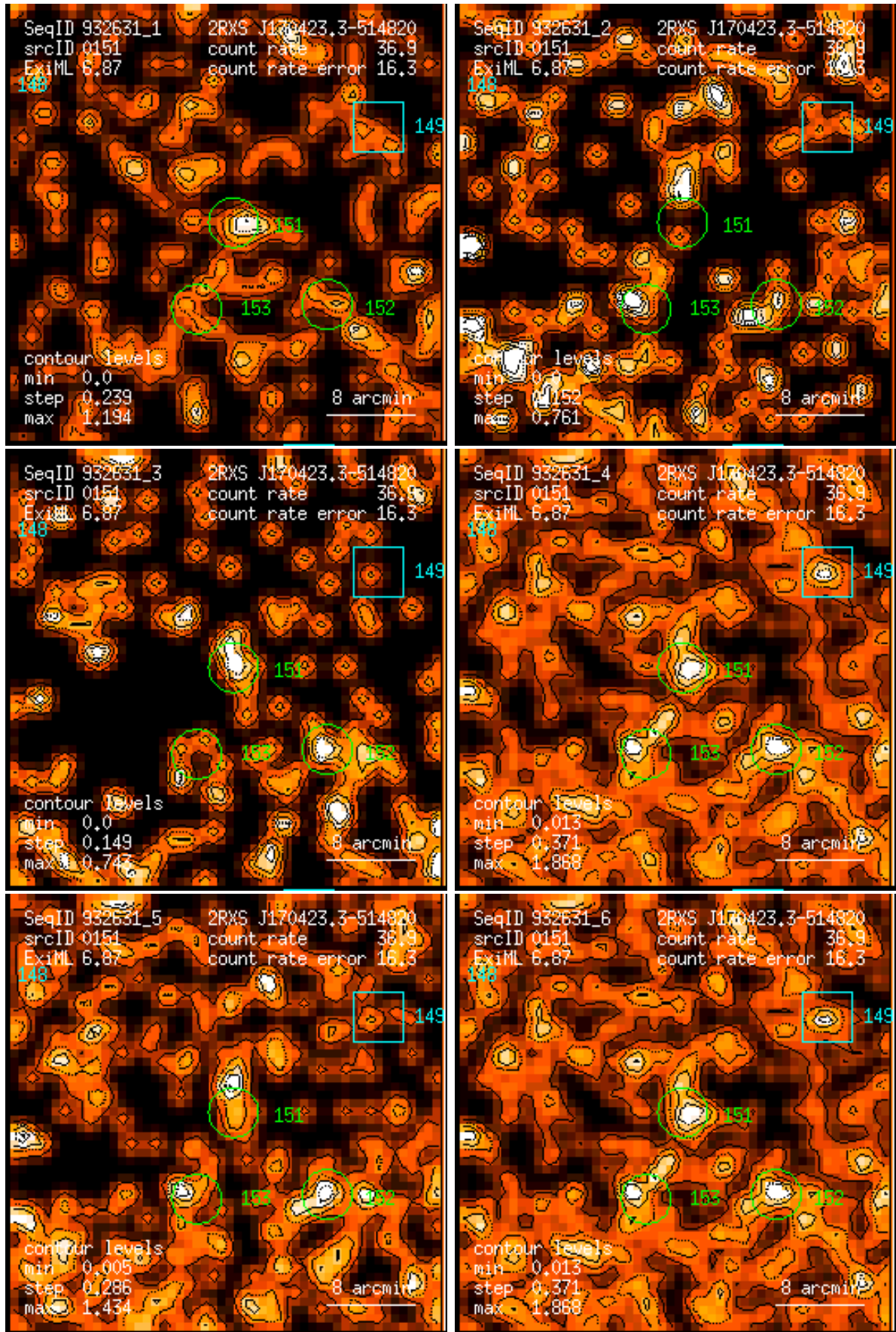
Figure 151: RASS 932631: detection 0151: band rate images, Gaussian filter: (1) PSPC channels 11 – 41, (2) 52 – 90, (3) 91 – 201, (4) 11 – 235, (5) 52 – 201, (6) 11 – 201. Broad band rates in counts/ks. Band rate contour levels in counts/ks/arcmin 2 .
