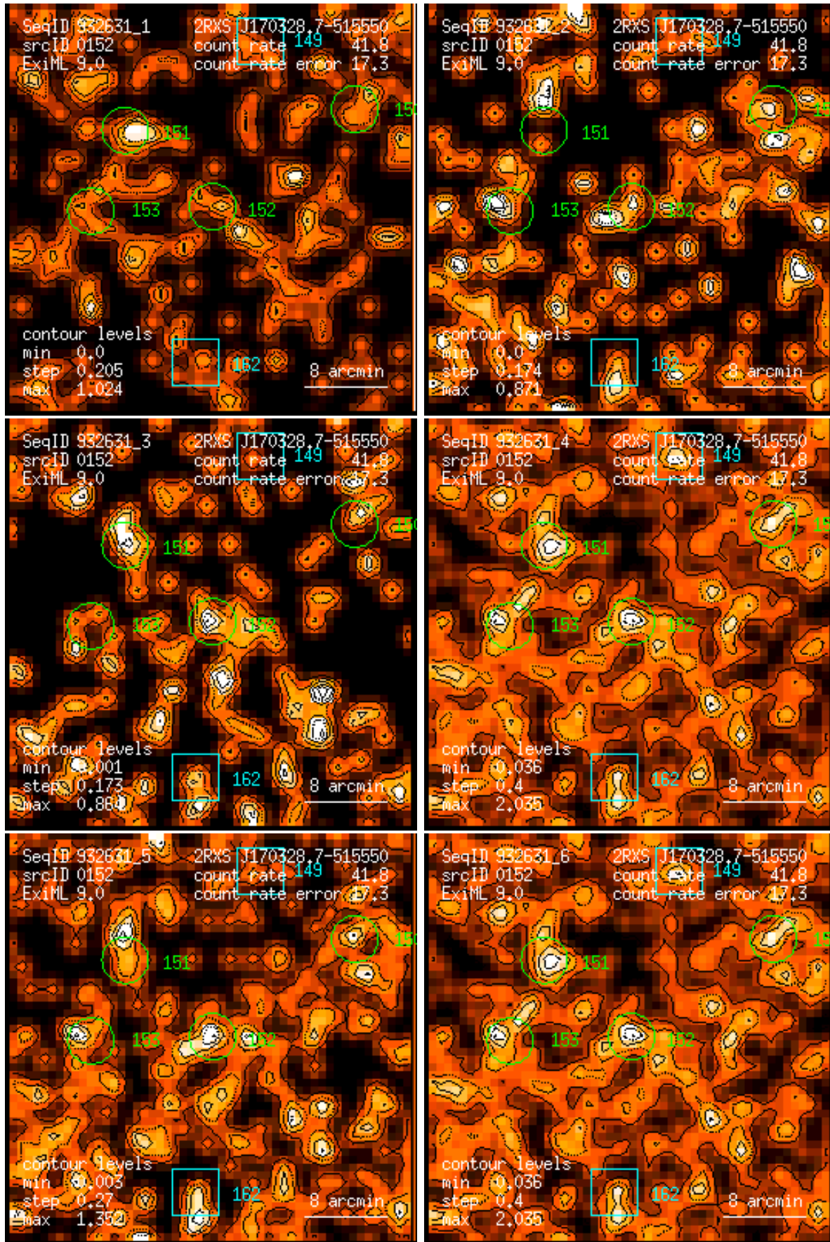
Figure 152: RASS 932631: detection 0152: band rate images, Gaussian filter: (1) PSPC channels 11 – 41, (2) 52 – 90, (3) 91 – 201, (4) 11 – 235, (5) 52 – 201, (6) 11 – 201. Broad band rates in counts/ks. Band rate contour levels in counts/ks/arcmin 2 .
