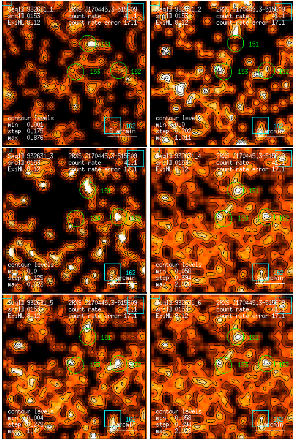
Figure 153: RASS 932631: detection 0153: band rate images, Gaussian filter: (1) PSPC channels 11 – 41, (2) 52 – 90, (3) 91 – 201, (4) 11 – 235, (5) 52 – 201, (6) 11 – 201. Broad band rates in counts/ks. Band rate contour levels in counts/ks/arcmin 2 .
