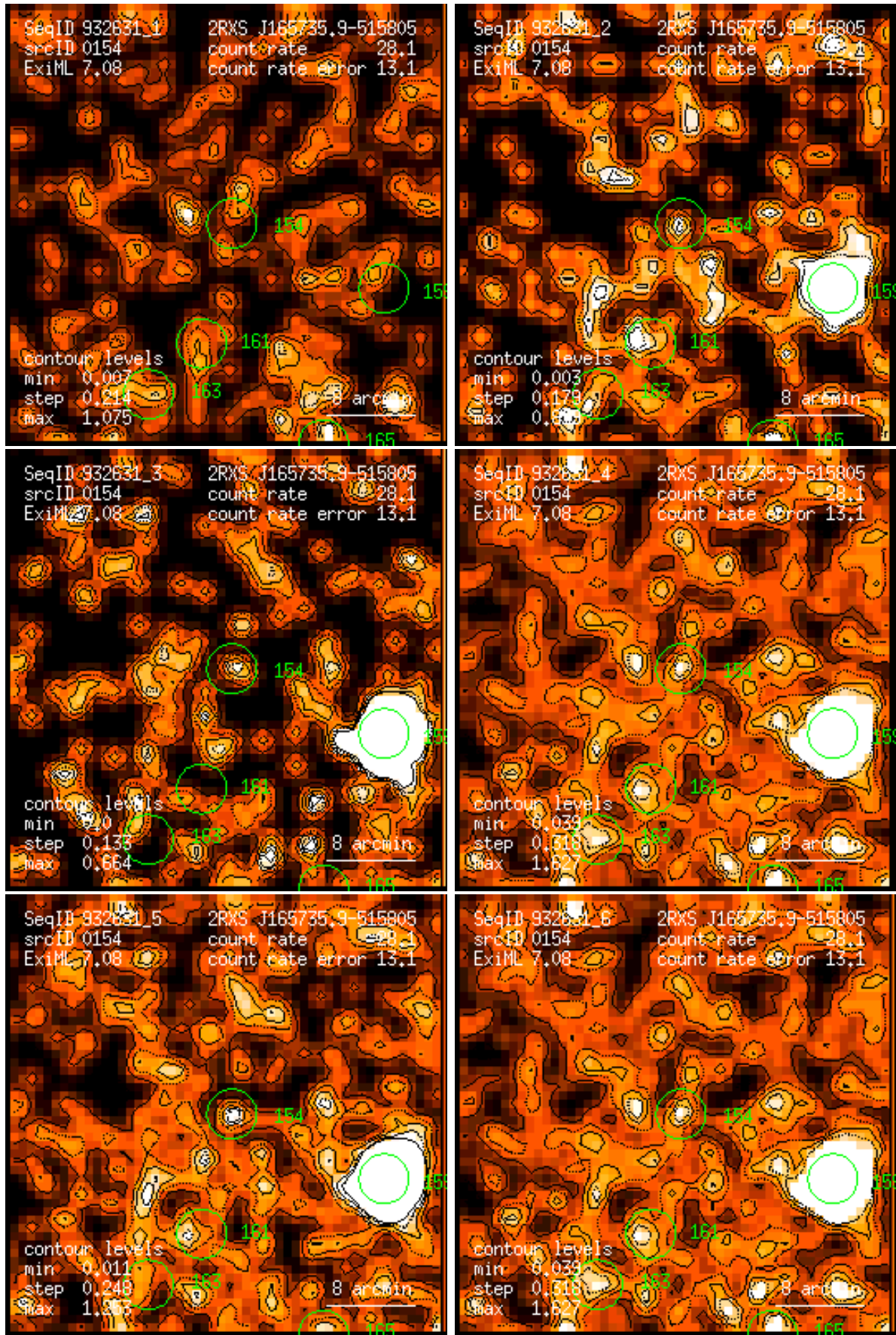
Figure 154: RASS 932631: detection 0154: band rate images, Gaussian filter: (1) PSPC channels 11 – 41, (2) 52 – 90, (3) 91 – 201, (4) 11 – 235, (5) 52 – 201, (6) 11 – 201. Broad band rates in counts/ks. Band rate contour levels in counts/ks/arcmin 2 .
