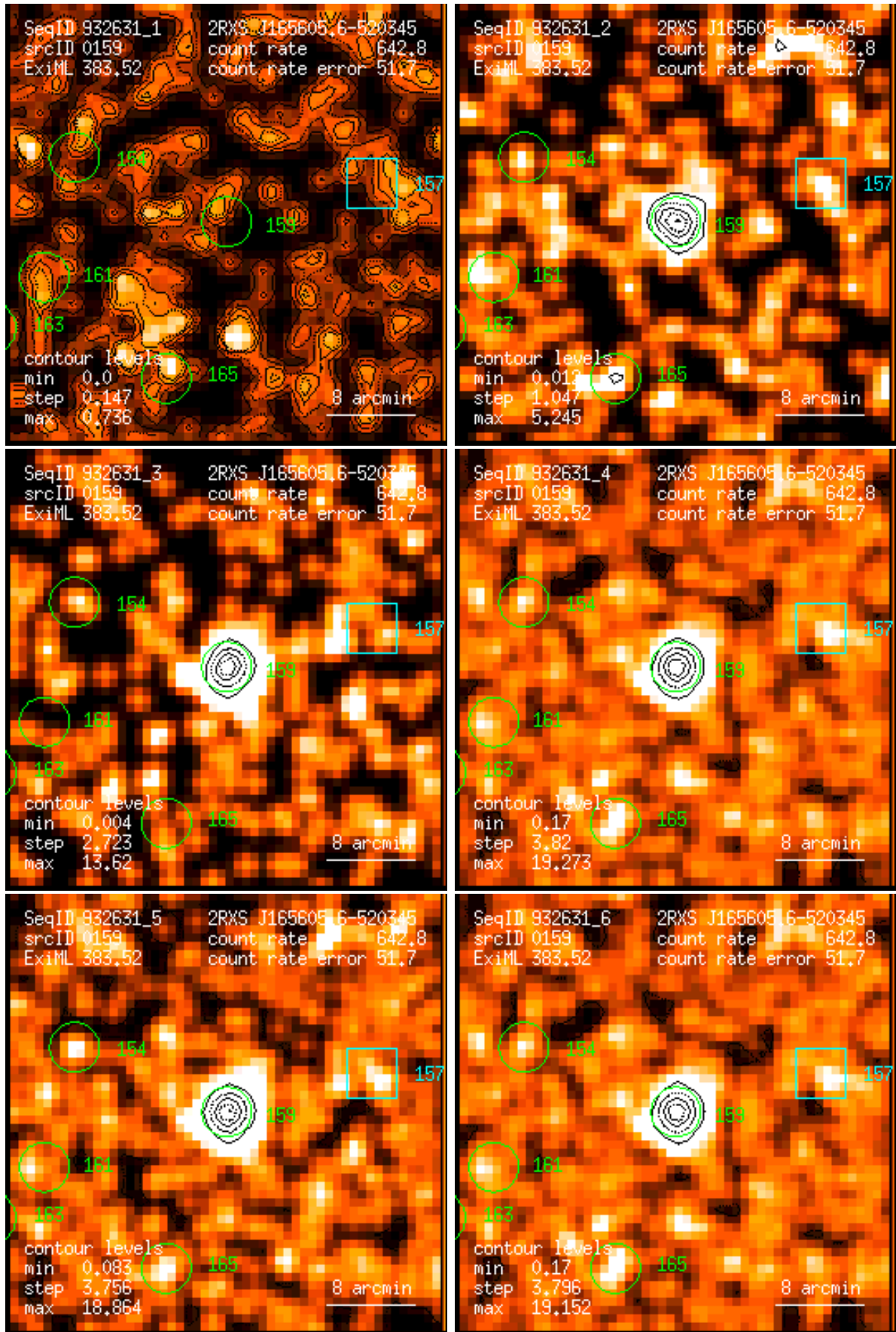
Figure 159: RASS 932631: detection 0159: band rate images, Gaussian filter: (1) PSPC channels 11 – 41, (2) 52 – 90, (3) 91 – 201, (4) 11 – 235, (5) 52 – 201, (6) 11 – 201. Broad band rates in counts/ks. Band rate contour levels in counts/ks/arcmin 2 .
