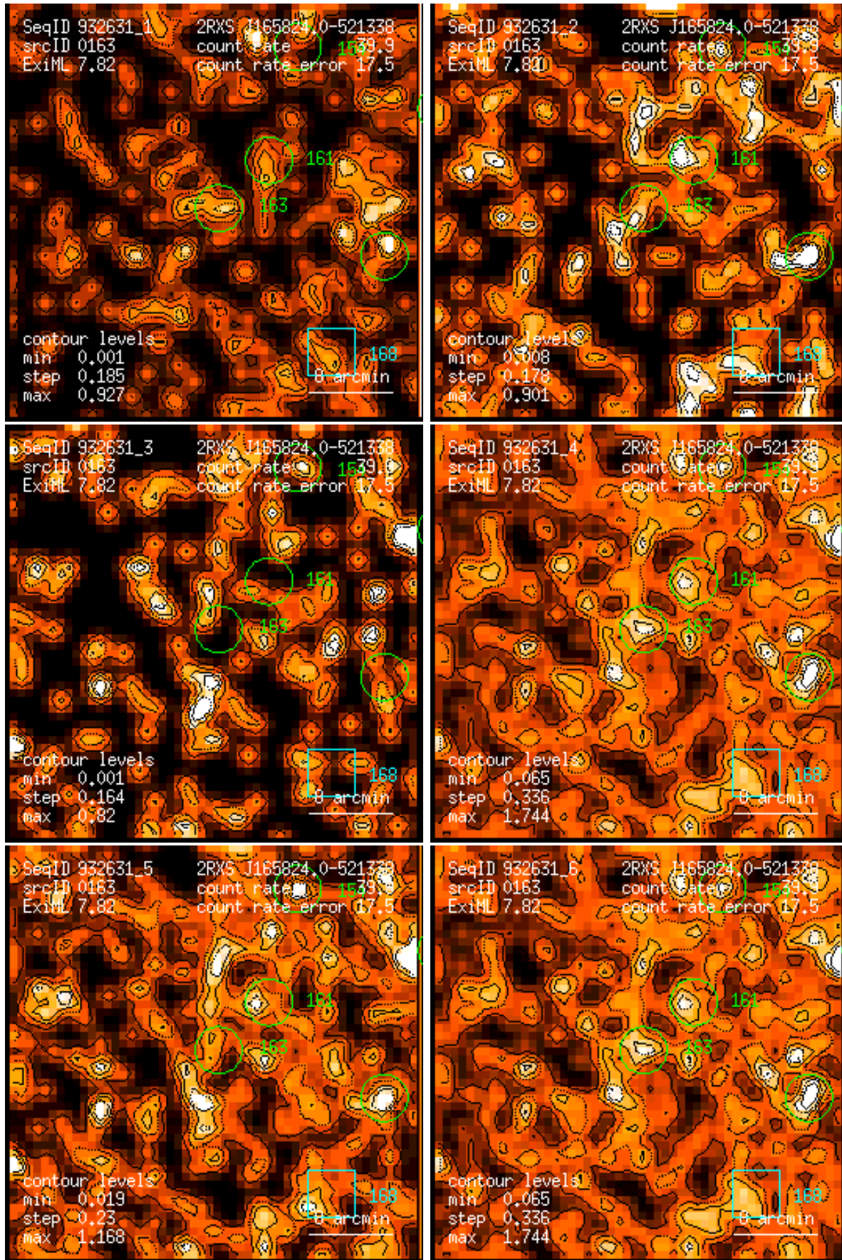
Figure 163: RASS 932631: detection 0163: band rate images, Gaussian filter: (1) PSPC channels 11 – 41, (2) 52 – 90, (3) 91 – 201, (4) 11 – 235, (5) 52 – 201, (6) 11 – 201. Broad band rates in counts/ks. Band rate contour levels in counts/ks/arcmin 2 .
