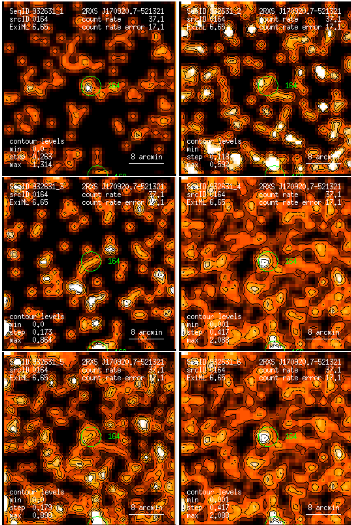
Figure 164: RASS 932631: detection 0164: band rate images, Gaussian filter: (1) PSPC channels 11 – 41, (2) 52 – 90, (3) 91 – 201, (4) 11 – 235, (5) 52 – 201, (6) 11 – 201. Broad band rates in counts/ks. Band rate contour levels in counts/ks/arcmin 2 .
