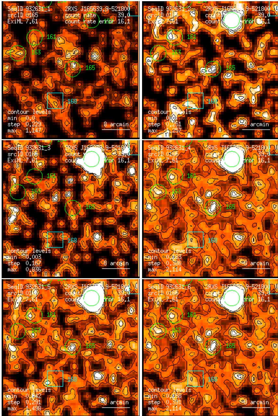
Figure 165: RASS 932631: detection 0165: band rate images, Gaussian filter: (1) PSPC channels 11 – 41, (2) 52 – 90, (3) 91 – 201, (4) 11 – 235, (5) 52 – 201, (6) 11 – 201. Broad band rates in counts/ks. Band rate contour levels in counts/ks/arcmin 2 .
