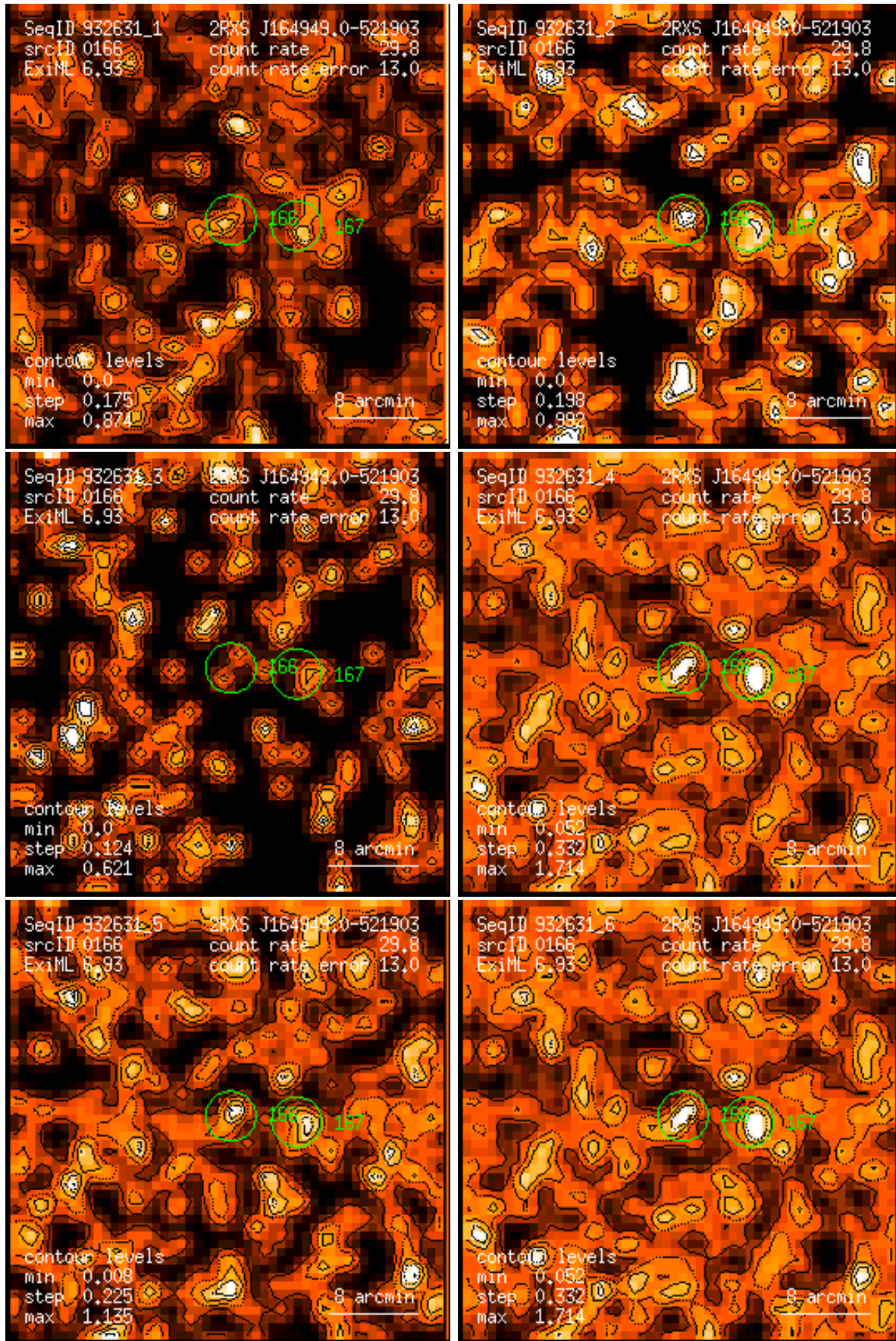
Figure 166: RASS 932631: detection 0166: band rate images, Gaussian filter: (1) PSPC channels 11 – 41, (2) 52 – 90, (3) 91 – 201, (4) 11 – 235, (5) 52 – 201, (6) 11 – 201. Broad band rates in counts/ks. Band rate contour levels in counts/ks/arcmin 2 .
