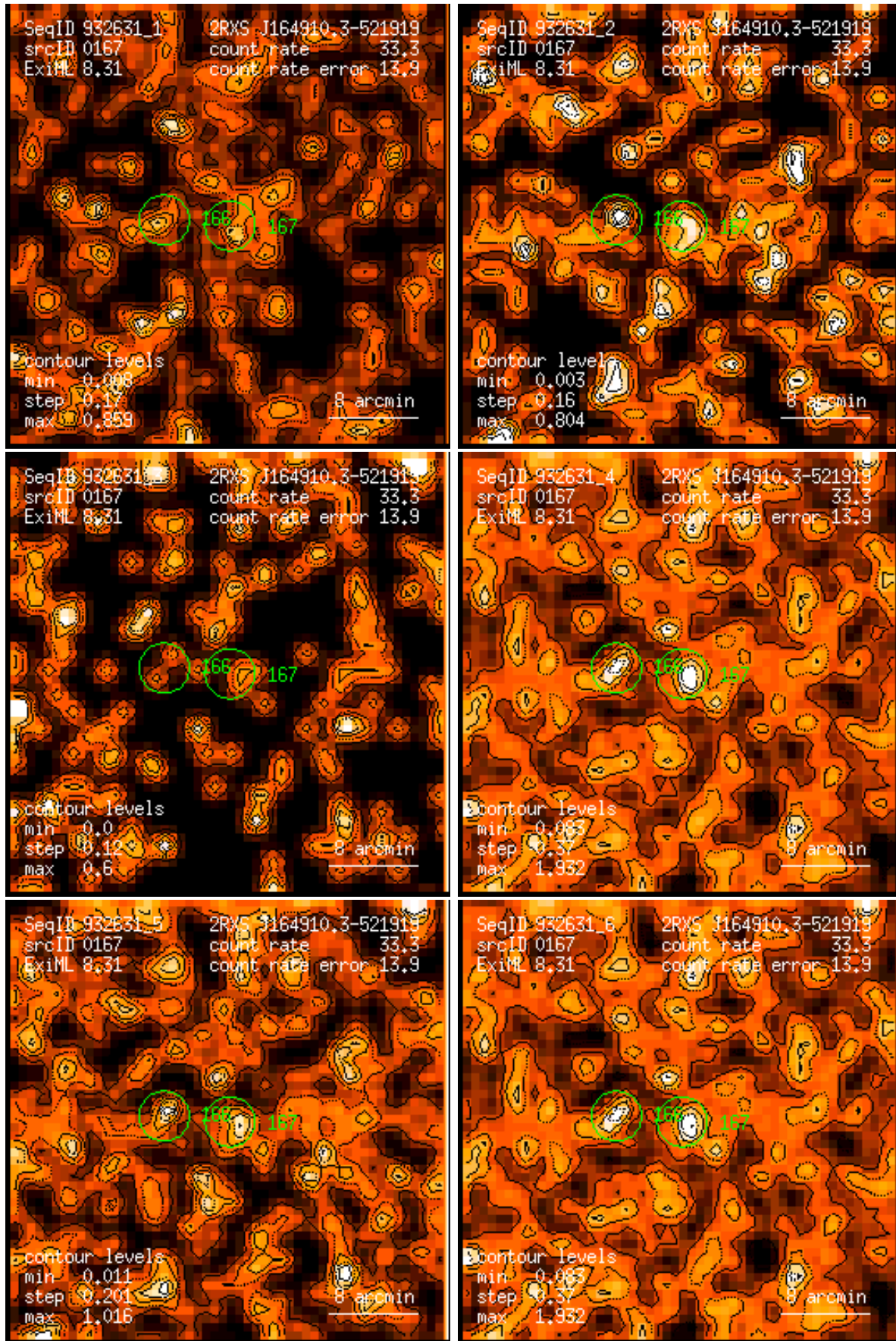
Figure 167: RASS 932631: detection 0167: band rate images, Gaussian filter: (1) PSPC channels 11 – 41, (2) 52 – 90, (3) 91 – 201, (4) 11 – 235, (5) 52 – 201, (6) 11 – 201. Broad band rates in counts/ks. Band rate contour levels in counts/ks/arcmin 2 .
