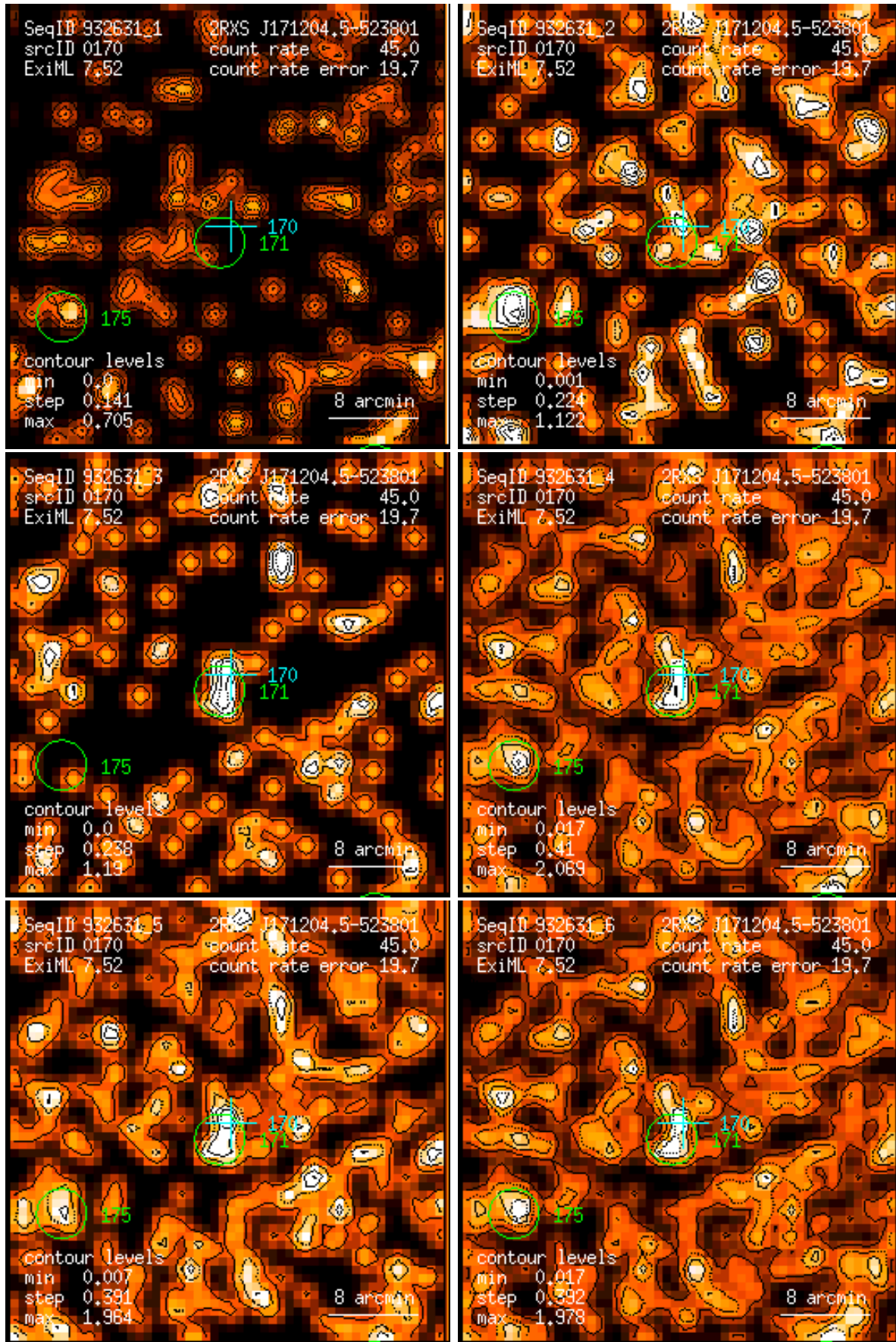
Figure 170: RASS 932631: detection 0170: band rate images, Gaussian filter: (1) PSPC channels 11 – 41, (2) 52 – 90, (3) 91 – 201, (4) 11 – 235, (5) 52 – 201, (6) 11 – 201. Broad band rates in counts/ks. Band rate contour levels in counts/ks/arcmin 2 .
