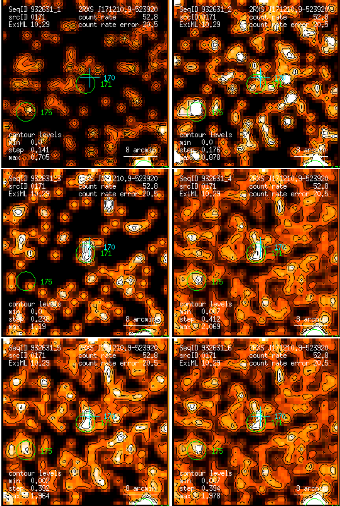
Figure 171: RASS 932631: detection 0171: band rate images, Gaussian filter: (1) PSPC channels 11 – 41, (2) 52 – 90, (3) 91 – 201, (4) 11 – 235, (5) 52 – 201, (6) 11 – 201. Broad band rates in counts/ks. Band rate contour levels in counts/ks/arcmin 2 .
