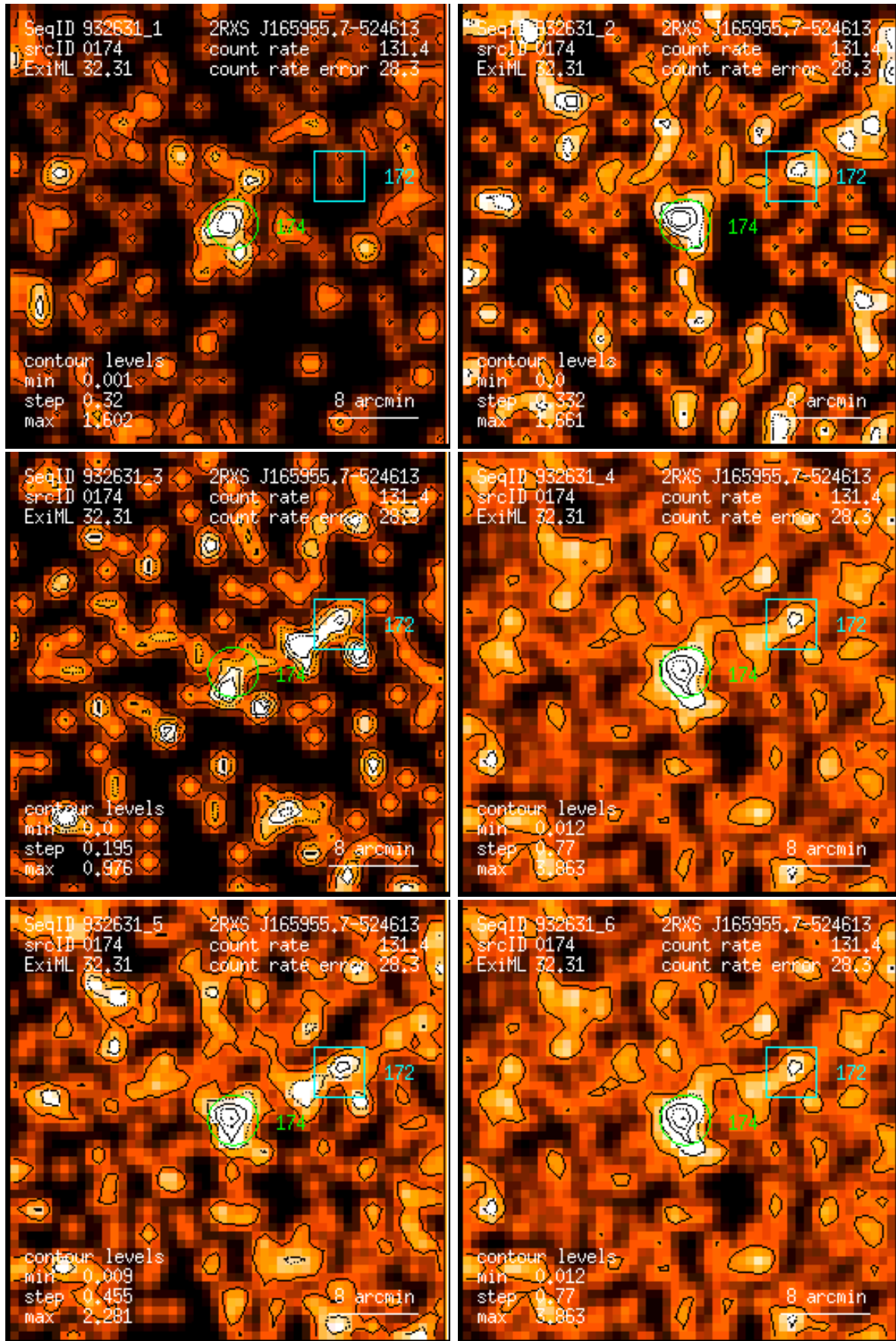
Figure 174: RASS 932631: detection 0174: band rate images, Gaussian filter: (1) PSPC channels 11 – 41, (2) 52 – 90, (3) 91 – 201, (4) 11 – 235, (5) 52 – 201, (6) 11 – 201. Broad band rates in counts/ks. Band rate contour levels in counts/ks/arcmin 2 .
