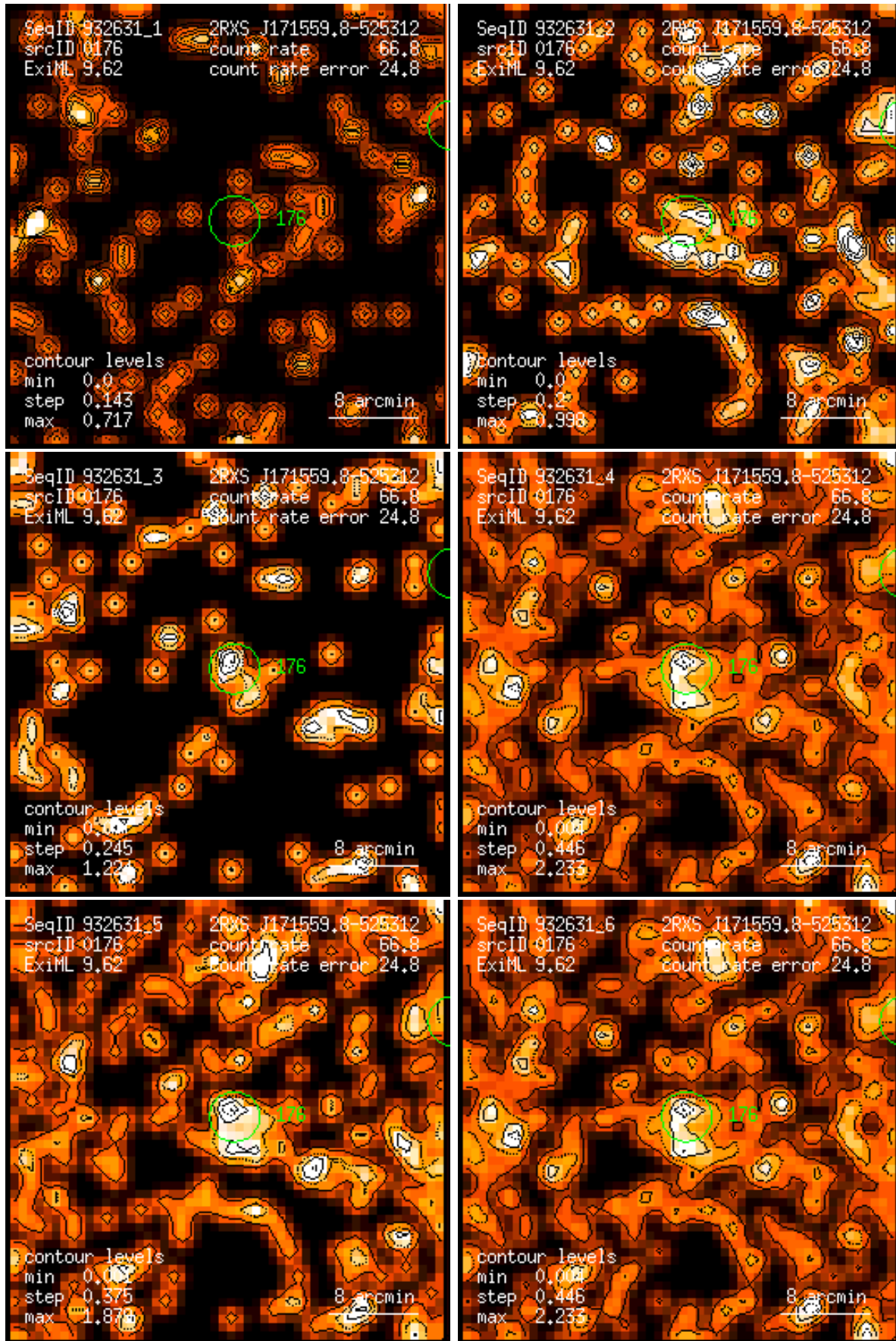
Figure 176: RASS 932631: detection 0176: band rate images, Gaussian filter: (1) PSPC channels 11 – 41, (2) 52 – 90, (3) 91 – 201, (4) 11 – 235, (5) 52 – 201, (6) 11 – 201. Broad band rates in counts/ks. Band rate contour levels in counts/ks/arcmin 2 .
