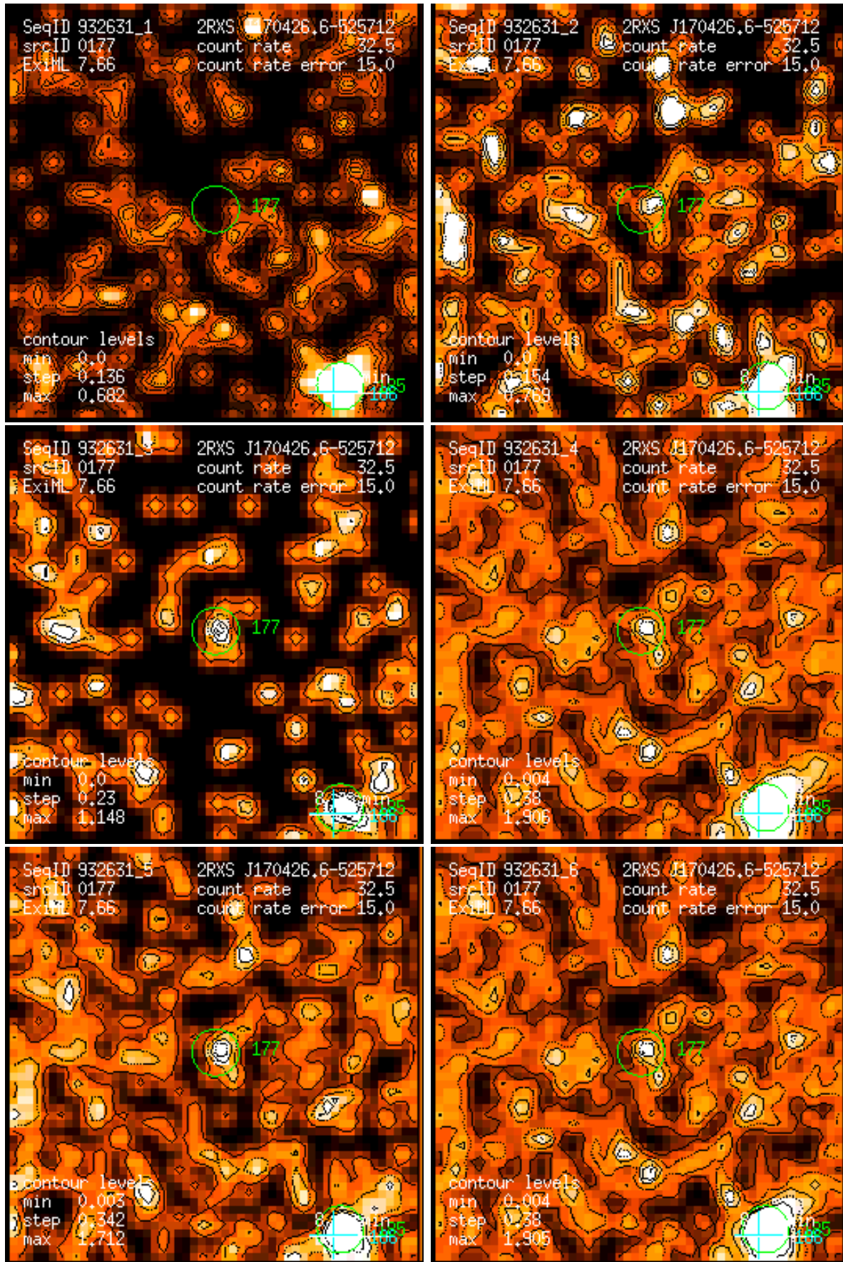
Figure 177: RASS 932631: detection 0177: band rate images, Gaussian filter: (1) PSPC channels 11 – 41, (2) 52 – 90, (3) 91 – 201, (4) 11 – 235, (5) 52 – 201, (6) 11 – 201. Broad band rates in counts/ks. Band rate contour levels in counts/ks/arcmin 2 .
