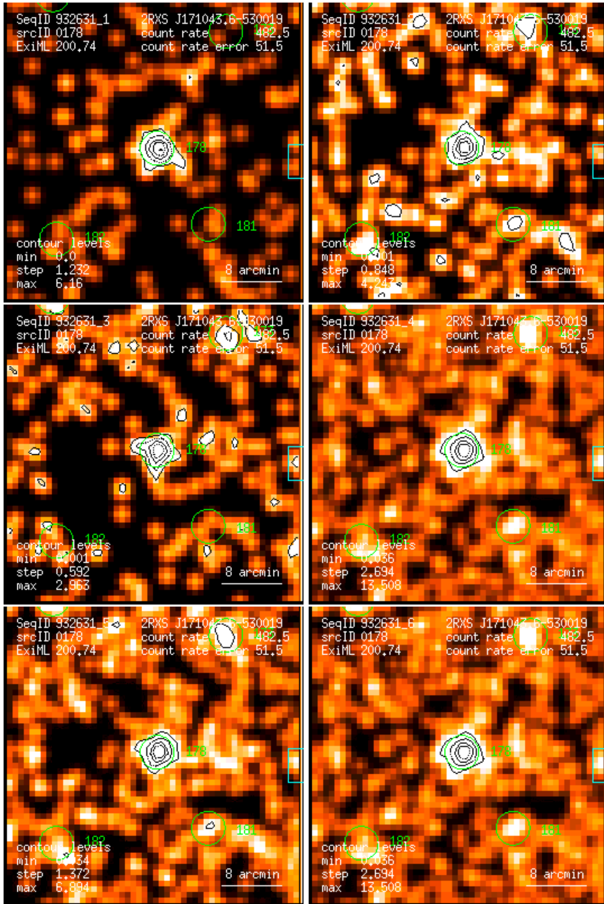
Figure 178: RASS 932631: detection 0178: band rate images, Gaussian filter: (1) PSPC channels 11 – 41, (2) 52 – 90, (3) 91 – 201, (4) 11 – 235, (5) 52 – 201, (6) 11 – 201. Broad band rates in counts/ks. Band rate contour levels in counts/ks/arcmin 2 .
