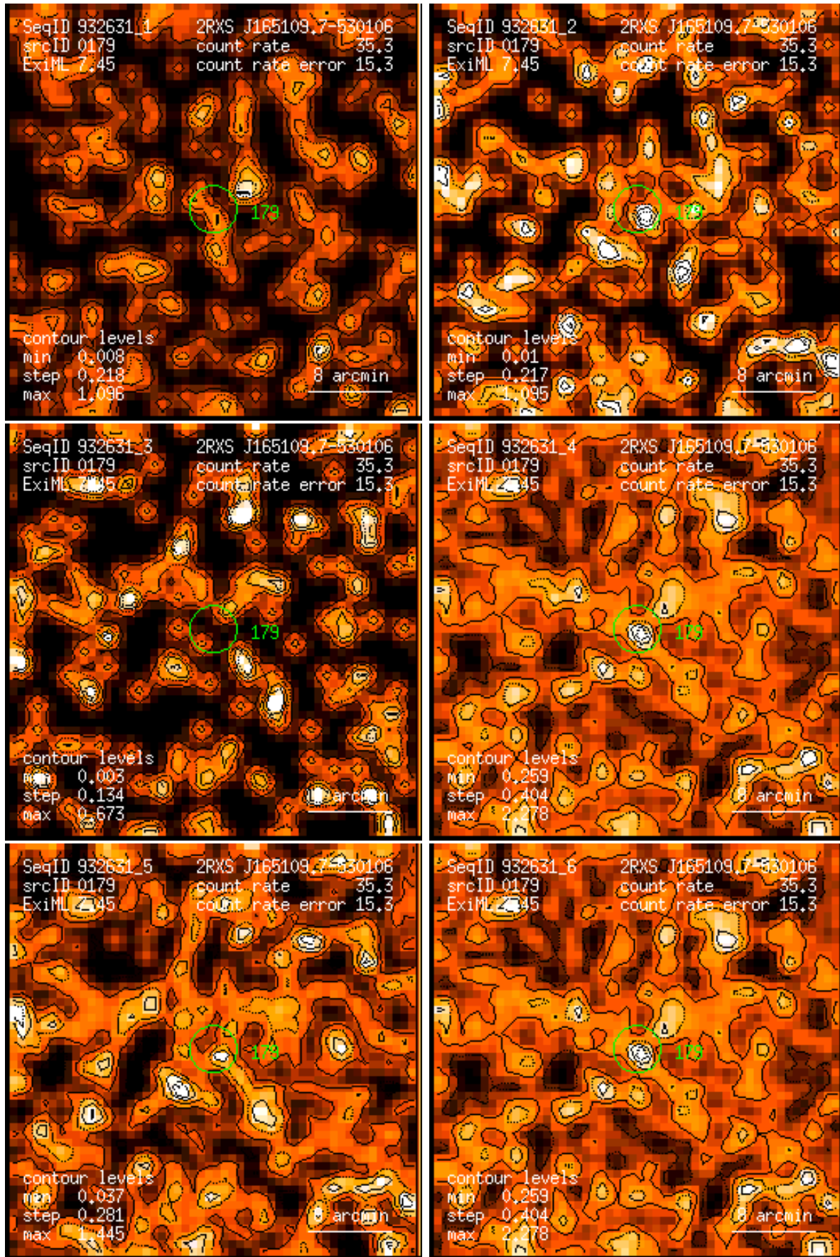
Figure 179: RASS 932631: detection 0179: band rate images, Gaussian filter: (1) PSPC channels 11 – 41, (2) 52 – 90, (3) 91 – 201, (4) 11 – 235, (5) 52 – 201, (6) 11 – 201. Broad band rates in counts/ks. Band rate contour levels in counts/ks/arcmin 2 .
