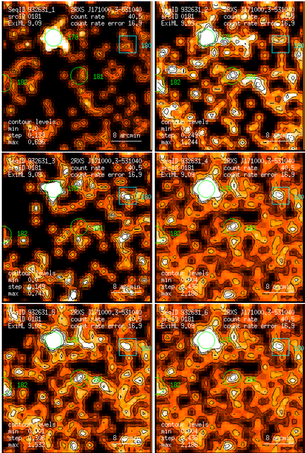
Figure 181: RASS 932631: detection 0181: band rate images, Gaussian filter: (1) PSPC channels 11 – 41, (2) 52 – 90, (3) 91 – 201, (4) 11 – 235, (5) 52 – 201, (6) 11 – 201. Broad band rates in counts/ks. Band rate contour levels in counts/ks/arcmin 2 .
