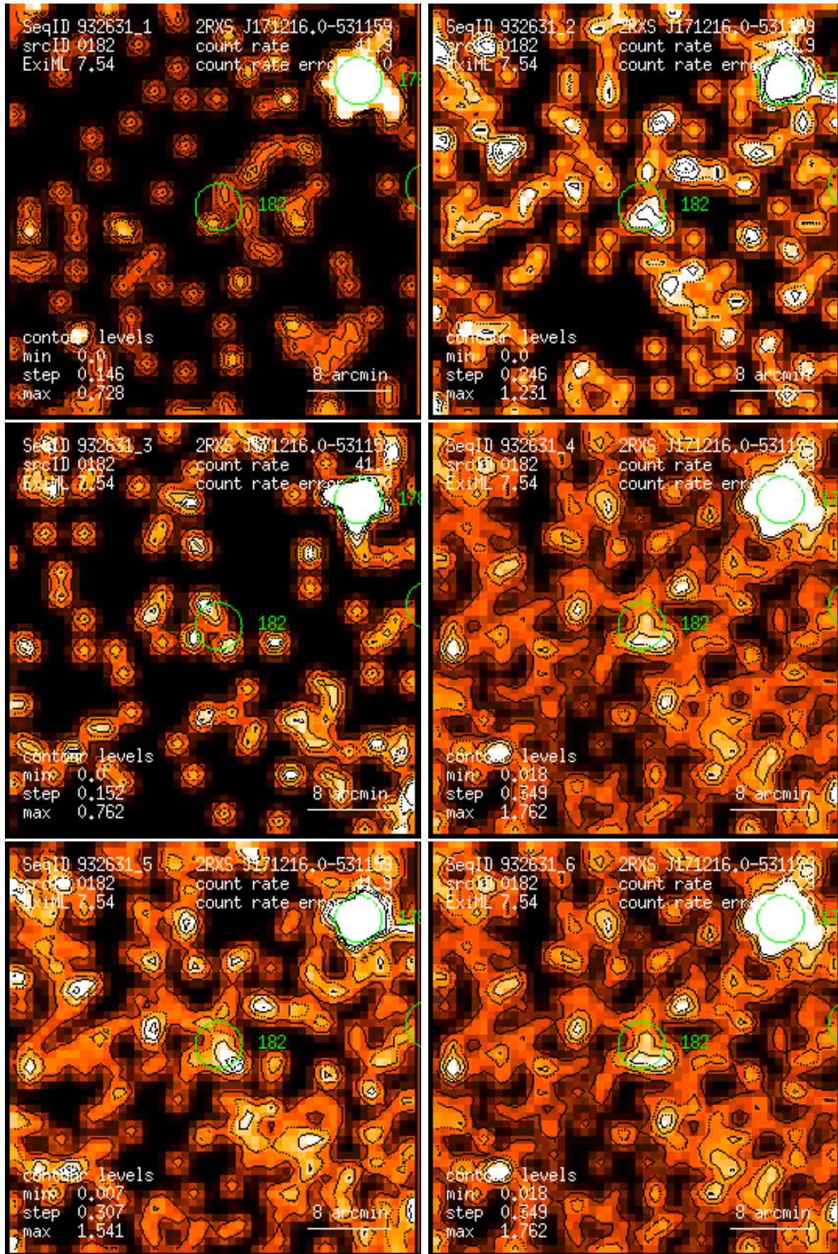
Figure 182: RASS 932631: detection 0182: band rate images, Gaussian filter: (1) PSPC channels 11 – 41, (2) 52 – 90, (3) 91 – 201, (4) 11 – 235, (5) 52 – 201, (6) 11 – 201. Broad band rates in counts/ks. Band rate contour levels in counts/ks/arcmin 2 .
