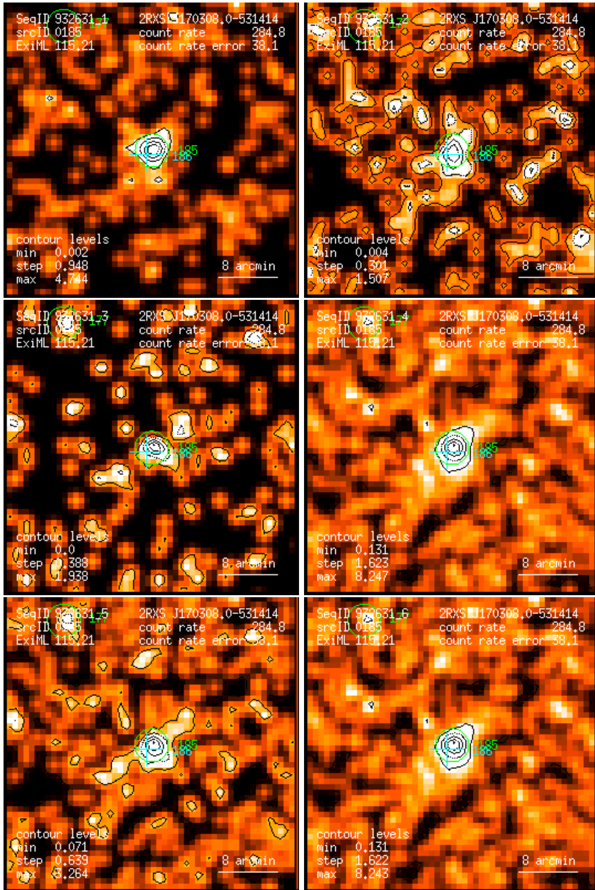
Figure 185: RASS 932631: detection 0185: band rate images, Gaussian filter: (1) PSPC channels 11 – 41, (2) 52 – 90, (3) 91 – 201, (4) 11 – 235, (5) 52 – 201, (6) 11 – 201. Broad band rates in counts/ks. Band rate contour levels in counts/ks/arcmin 2 .
