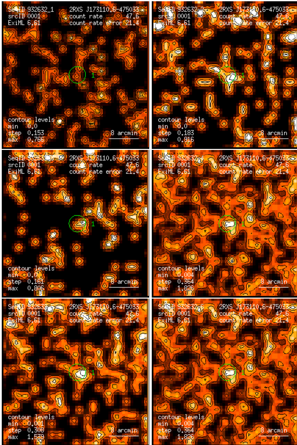
Figure 1: RASS 932632: detection 0001: band rate images, Gaussian filter: (1) PSPC channels 11 – 41, (2) 52 – 90, (3) 91 – 201, (4) 11 – 235, (5) 52 – 201, (6) 11 – 201. Broad band rates in counts/ks. Band rate contour levels in counts/ks/arcmin 2 .
