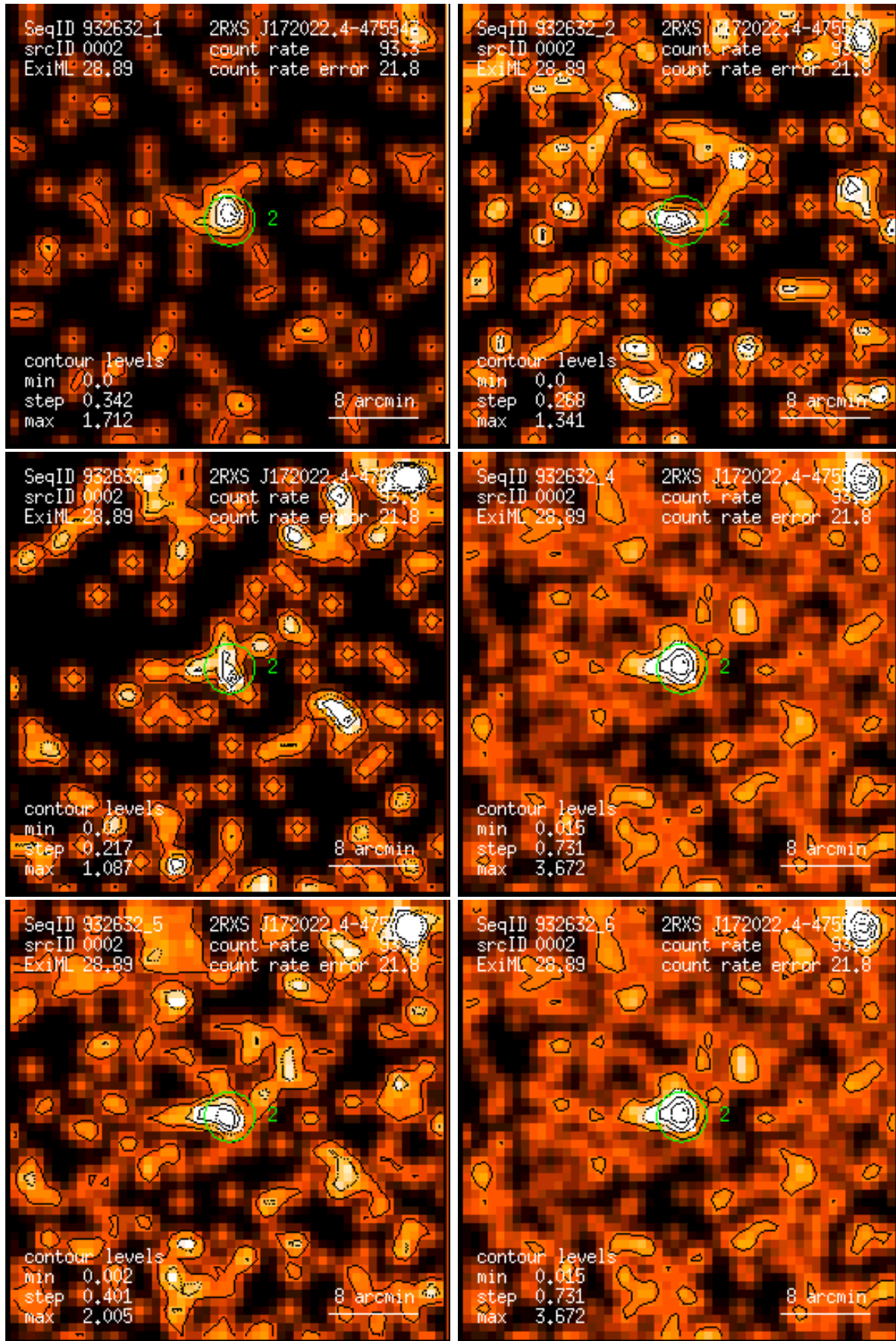
Figure 2: RASS 932632: detection 0002: band rate images, Gaussian filter: (1) PSPC channels 11 – 41, (2) 52 – 90, (3) 91 – 201, (4) 11 – 235, (5) 52 – 201, (6) 11 – 201. Broad band rates in counts/ks. Band rate contour levels in counts/ks/arcmin 2 .
