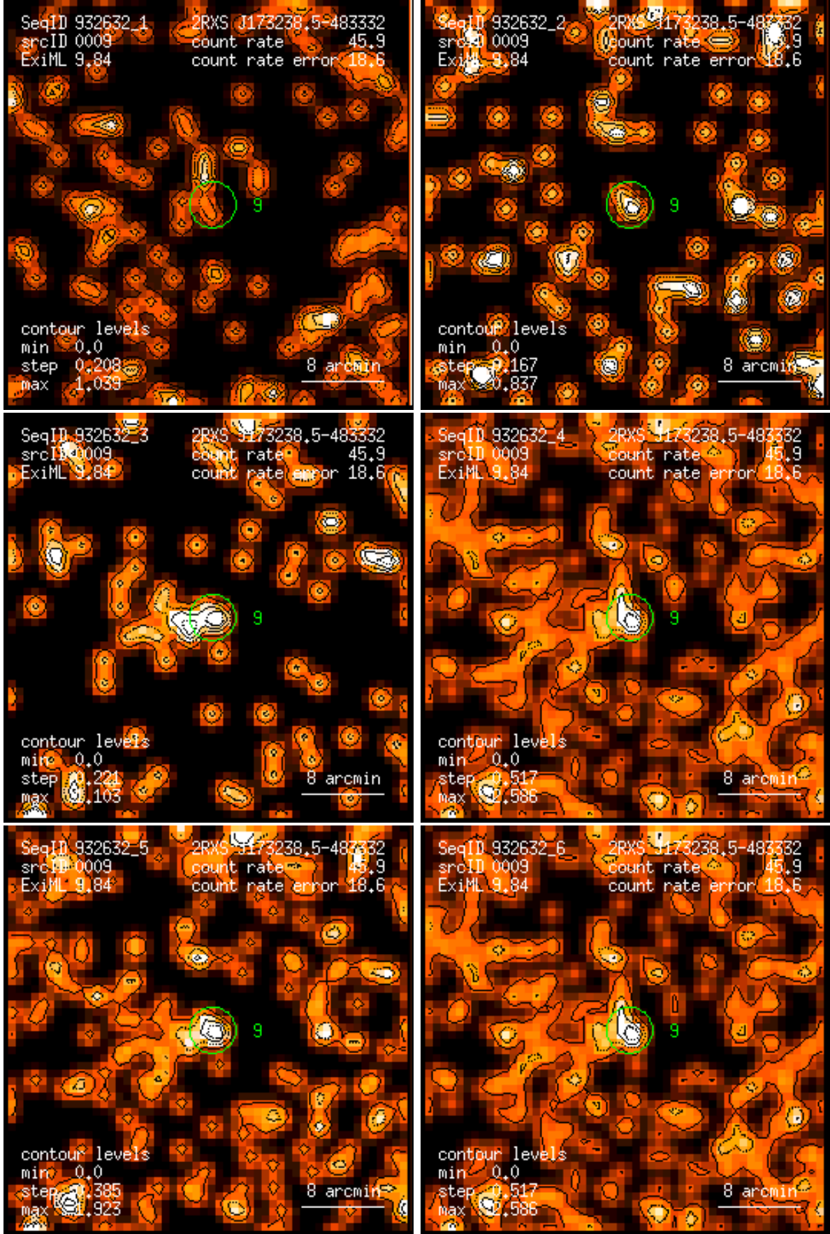
Figure 9: RASS 932632: detection 0009: band rate images, Gaussian filter: (1) PSPC channels 11 – 41, (2) 52 – 90, (3) 91 – 201, (4) 11 – 235, (5) 52 – 201, (6) 11 – 201. Broad band rates in counts/ks. Band rate contour levels in counts/ks/arcmin 2 .
