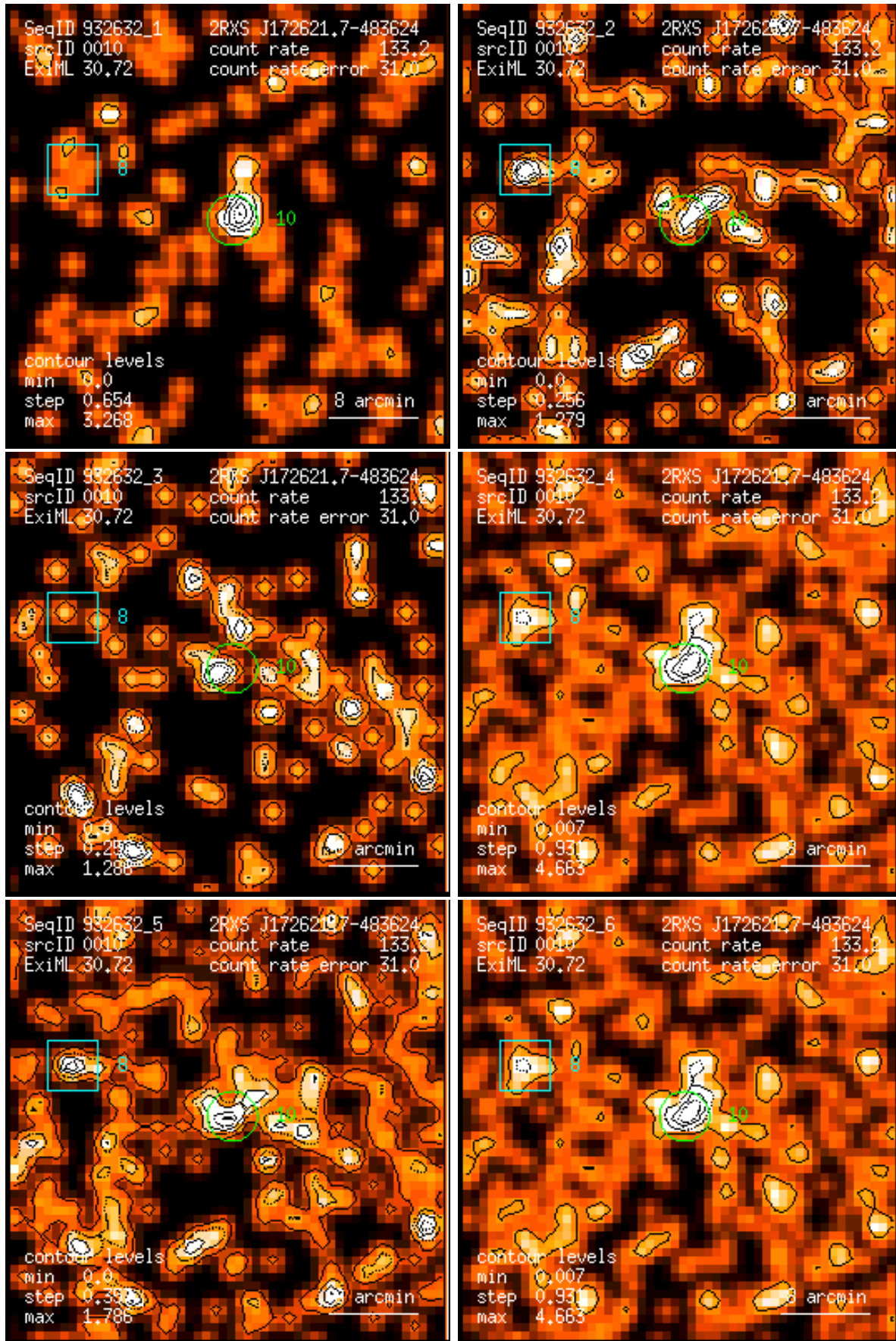
Figure 10: RASS 932632: detection 0010: band rate images, Gaussian filter: (1) PSPC channels 11 – 41, (2) 52 – 90, (3) 91 – 201, (4) 11 – 235, (5) 52 – 201, (6) 11 – 201. Broad band rates in counts/ks. Band rate contour levels in counts/ks/arcmin 2 .
