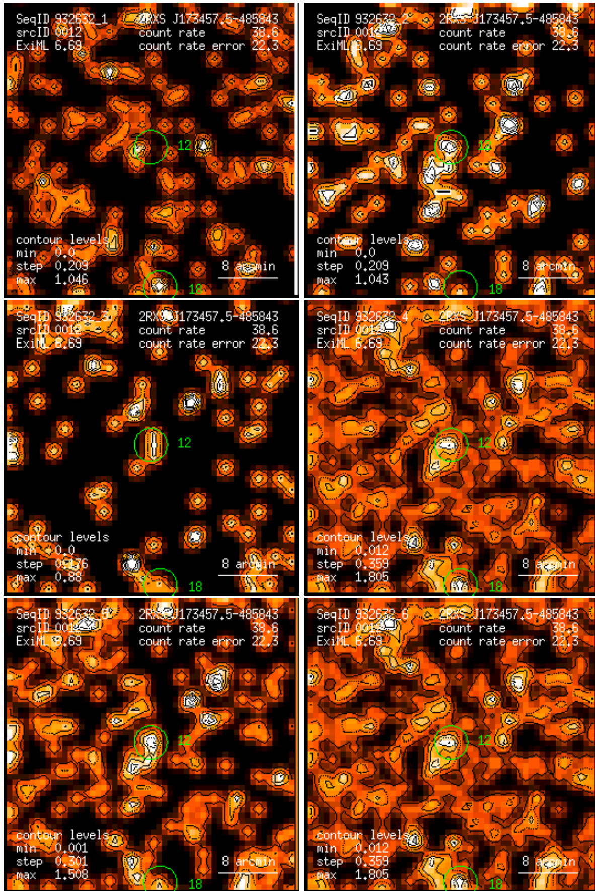
Figure 12: RASS 932632: detection 0012: band rate images, Gaussian filter: (1) PSPC channels 11 – 41, (2) 52 – 90, (3) 91 – 201, (4) 11 – 235, (5) 52 – 201, (6) 11 – 201. Broad band rates in counts/ks. Band rate contour levels in counts/ks/arcmin 2 .
