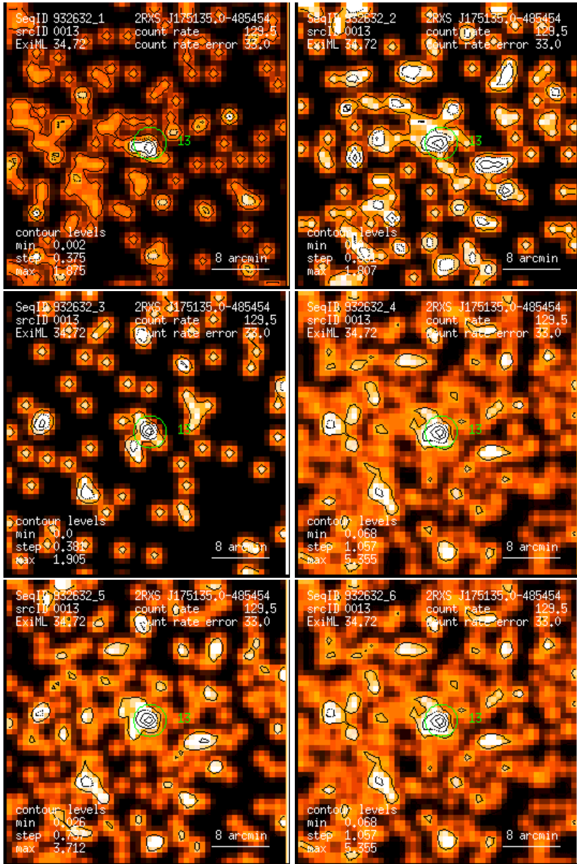
Figure 13: RASS 932632: detection 0013: band rate images, Gaussian filter: (1) PSPC channels 11 – 41, (2) 52 – 90, (3) 91 – 201, (4) 11 – 235, (5) 52 – 201, (6) 11 – 201. Broad band rates in counts/ks. Band rate contour levels in counts/ks/arcmin 2 .
