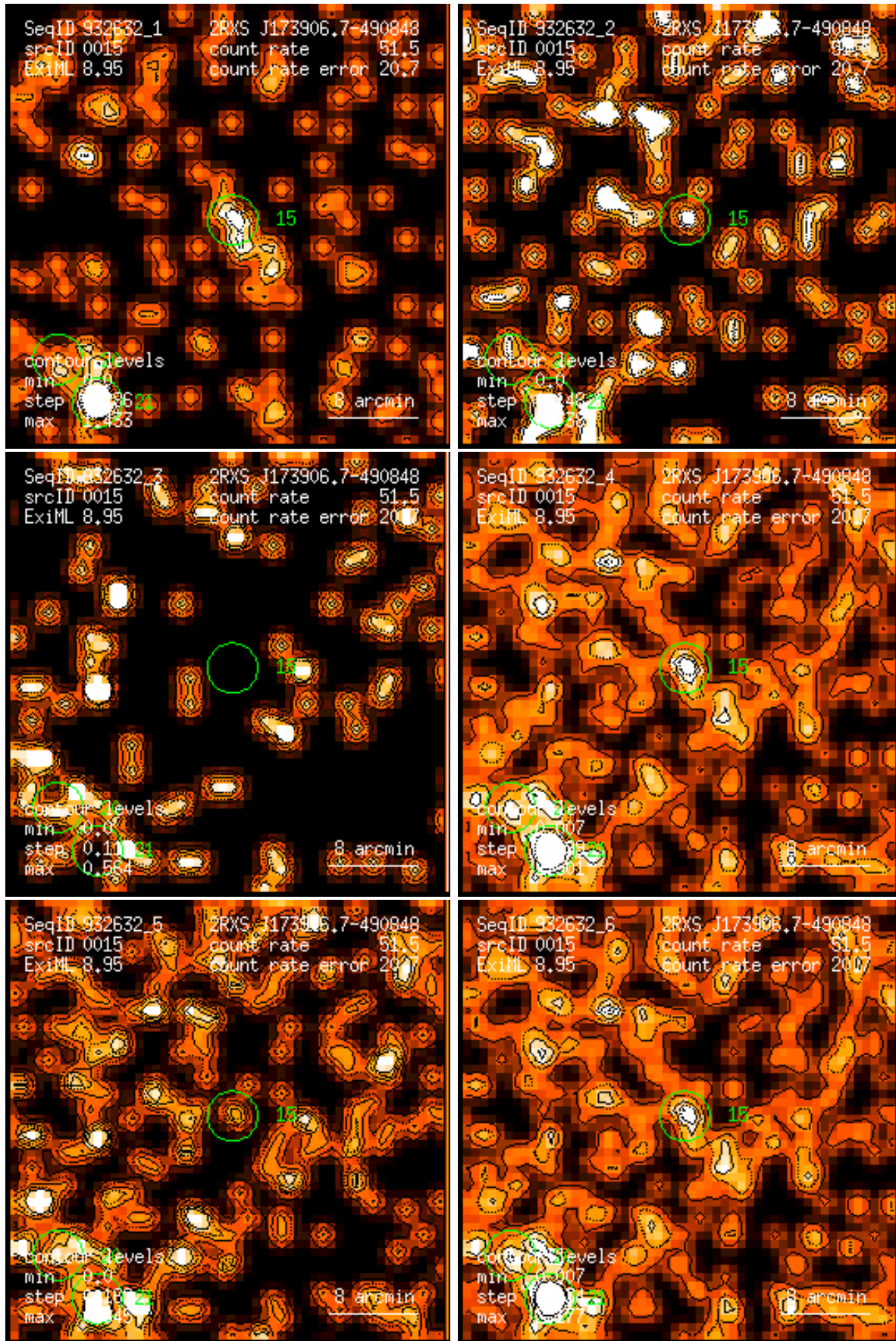
Figure 15: RASS 932632: detection 0015: band rate images, Gaussian filter: (1) PSPC channels 11 – 41, (2) 52 – 90, (3) 91 – 201, (4) 11 – 235, (5) 52 – 201, (6) 11 – 201. Broad band rates in counts/ks. Band rate contour levels in counts/ks/arcmin 2 .
