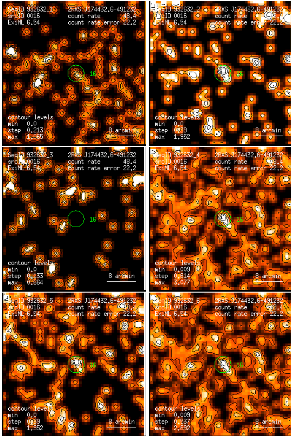
Figure 16: RASS 932632: detection 0016: band rate images, Gaussian filter: (1) PSPC channels 11 – 41, (2) 52 – 90, (3) 91 – 201, (4) 11 – 235, (5) 52 – 201, (6) 11 – 201. Broad band rates in counts/ks. Band rate contour levels in counts/ks/arcmin 2 .
