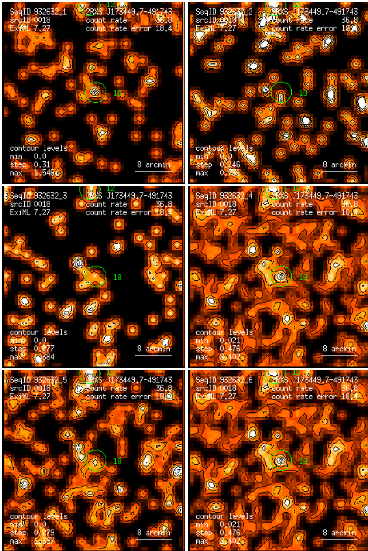
Figure 18: RASS 932632: detection 0018: band rate images, Gaussian filter: (1) PSPC channels 11 – 41, (2) 52 – 90, (3) 91 – 201, (4) 11 – 235, (5) 52 – 201, (6) 11 – 201. Broad band rates in counts/ks. Band rate contour levels in counts/ks/arcmin 2 .
