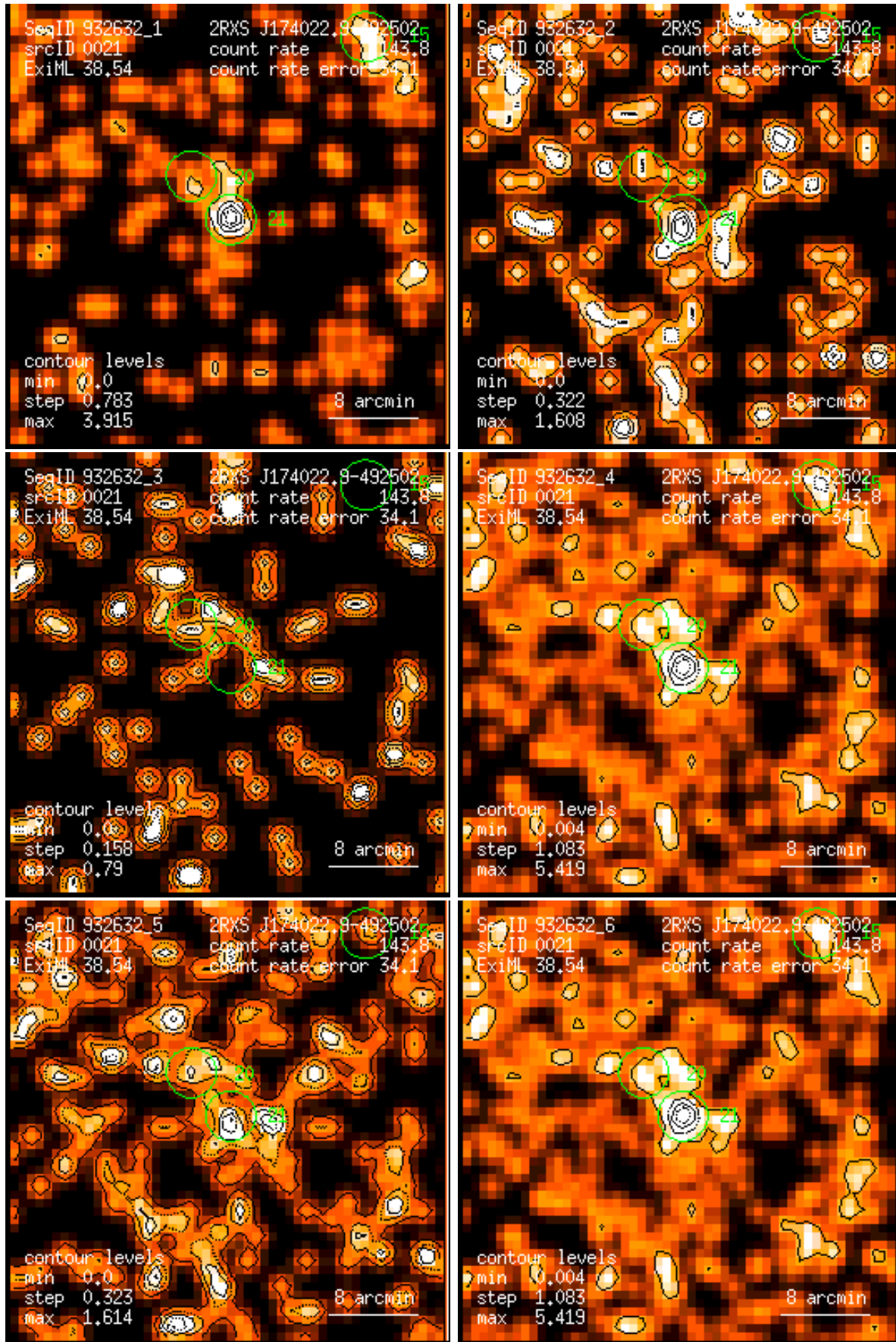
Figure 21: RASS 932632: detection 0021: band rate images, Gaussian filter: (1) PSPC channels 11 – 41, (2) 52 – 90, (3) 91 – 201, (4) 11 – 235, (5) 52 – 201, (6) 11 – 201. Broad band rates in counts/ks. Band rate contour levels in counts/ks/arcmin 2 .
