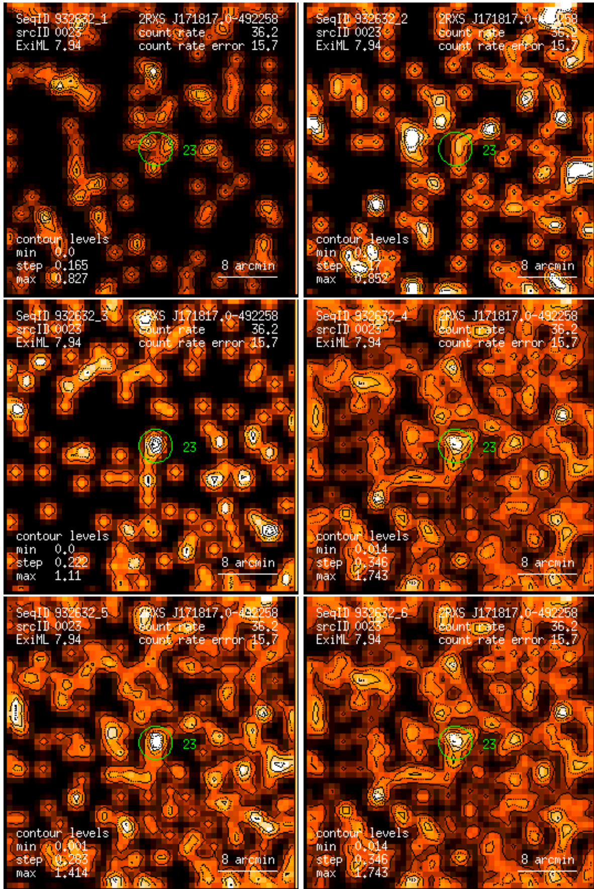
Figure 23: RASS 932632: detection 0023: band rate images, Gaussian filter: (1) PSPC channels 11 – 41, (2) 52 – 90, (3) 91 – 201, (4) 11 – 235, (5) 52 – 201, (6) 11 – 201. Broad band rates in counts/ks. Band rate contour levels in counts/ks/arcmin 2 .
