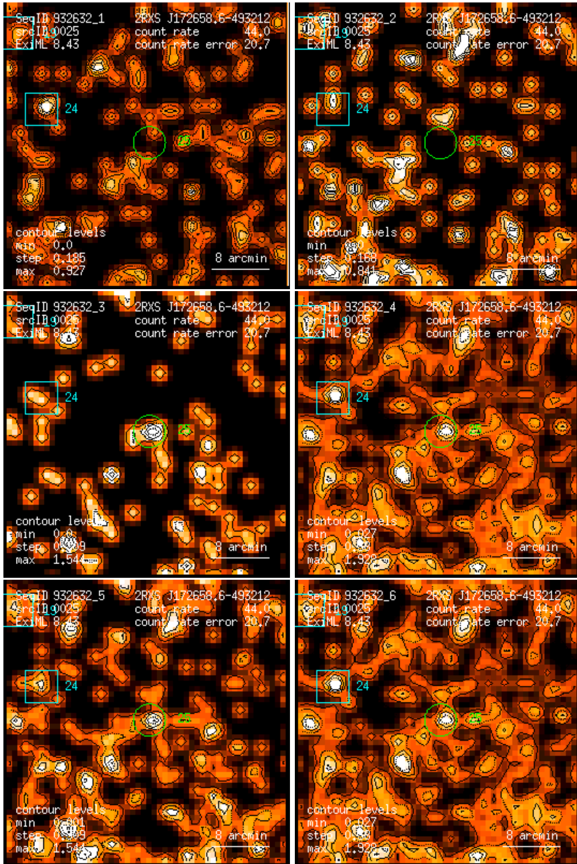
Figure 25: RASS 932632: detection 0025: band rate images, Gaussian filter: (1) PSPC channels 11 – 41, (2) 52 – 90, (3) 91 – 201, (4) 11 – 235, (5) 52 – 201, (6) 11 – 201. Broad band rates in counts/ks. Band rate contour levels in counts/ks/arcmin 2 .
