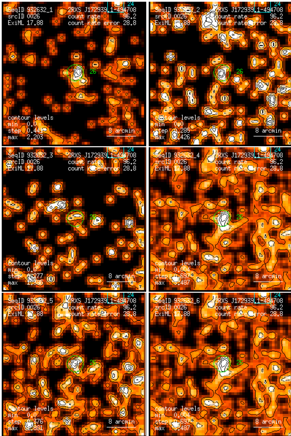
Figure 26: RASS 932632: detection 0026: band rate images, Gaussian filter: (1) PSPC channels 11 – 41, (2) 52 – 90, (3) 91 – 201, (4) 11 – 235, (5) 52 – 201, (6) 11 – 201. Broad band rates in counts/ks. Band rate contour levels in counts/ks/arcmin 2 .
