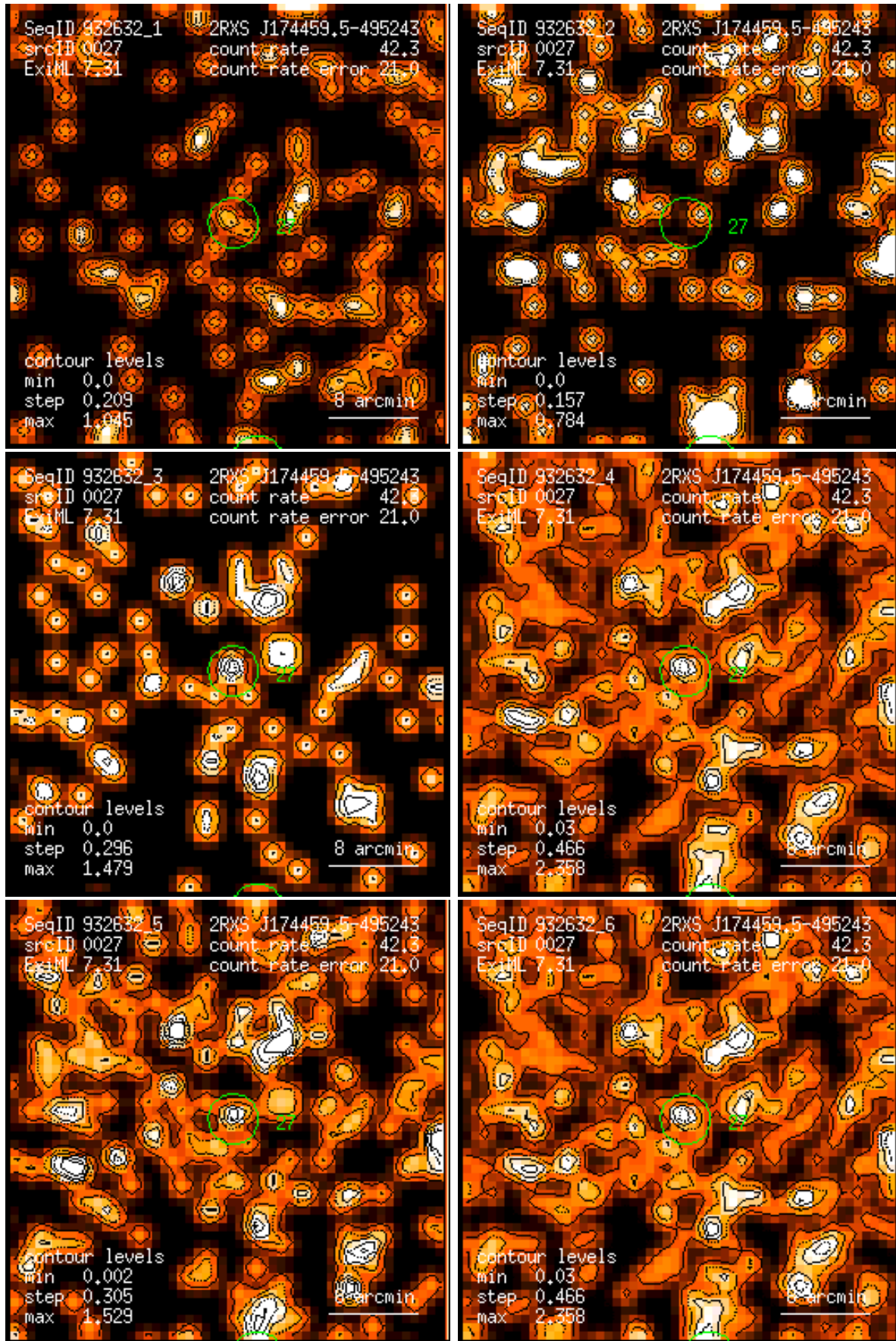
Figure 27: RASS 932632: detection 0027: band rate images, Gaussian filter: (1) PSPC channels 11 – 41, (2) 52 – 90, (3) 91 – 201, (4) 11 – 235, (5) 52 – 201, (6) 11 – 201. Broad band rates in counts/ks. Band rate contour levels in counts/ks/arcmin 2 .
