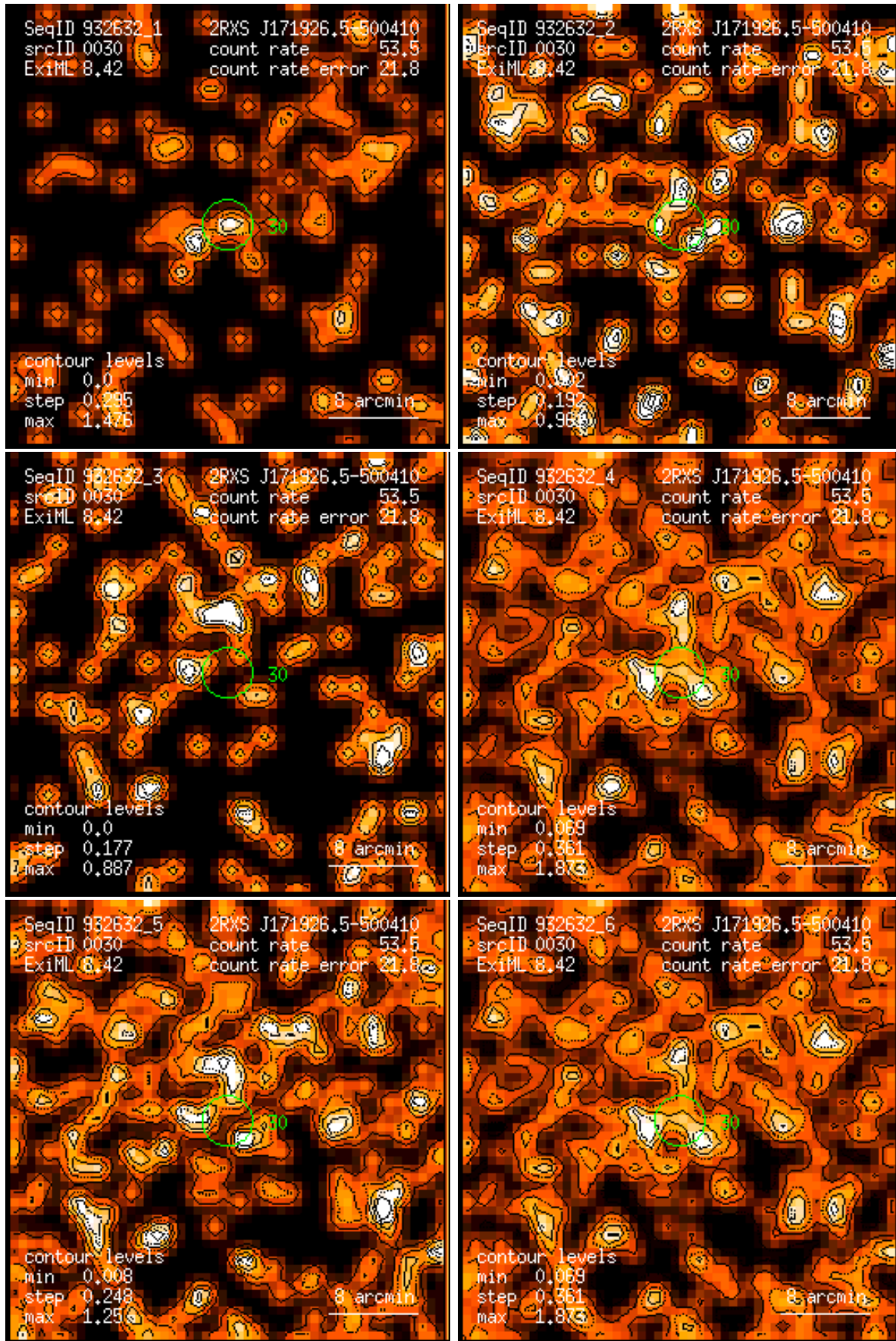
Figure 30: RASS 932632: detection 0030: band rate images, Gaussian filter: (1) PSPC channels 11 – 41, (2) 52 – 90, (3) 91 – 201, (4) 11 – 235, (5) 52 – 201, (6) 11 – 201. Broad band rates in counts/ks. Band rate contour levels in counts/ks/arcmin 2 .
