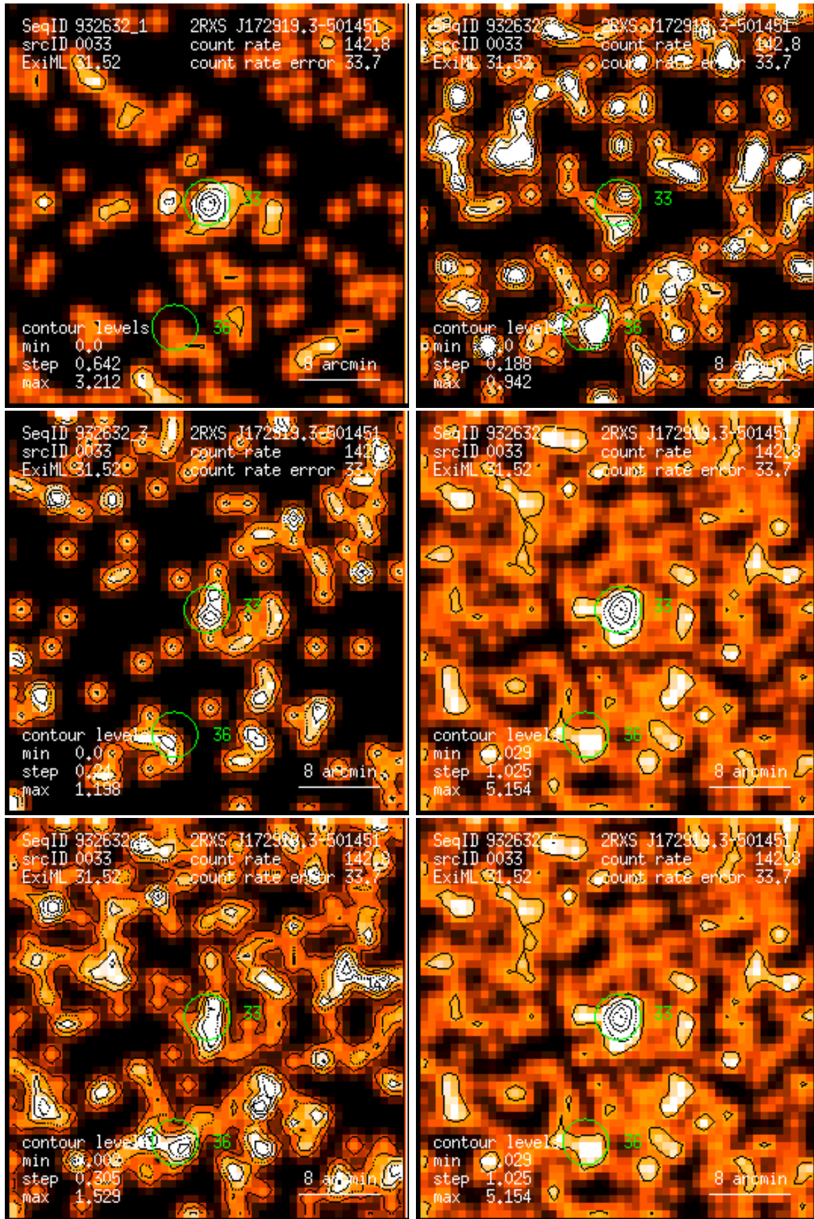
Figure 33: RASS 932632: detection 0033: band rate images, Gaussian filter: (1) PSPC channels 11 – 41, (2) 52 – 90, (3) 91 – 201, (4) 11 – 235, (5) 52 – 201, (6) 11 – 201. Broad band rates in counts/ks. Band rate contour levels in counts/ks/arcmin 2 .
