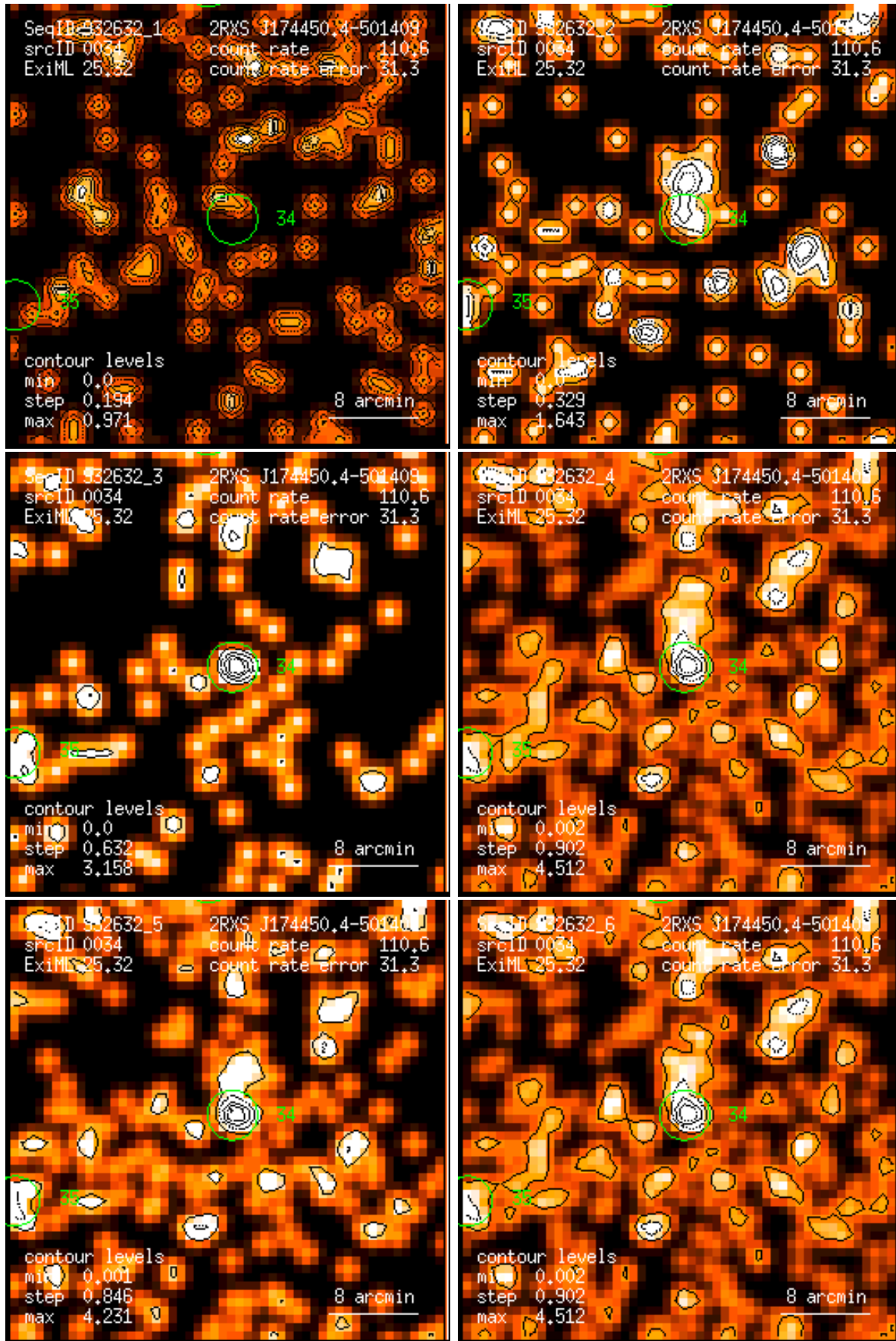
Figure 34: RASS 932632: detection 0034: band rate images, Gaussian filter: (1) PSPC channels 11 – 41, (2) 52 – 90, (3) 91 – 201, (4) 11 – 235, (5) 52 – 201, (6) 11 – 201. Broad band rates in counts/ks. Band rate contour levels in counts/ks/arcmin 2 .
