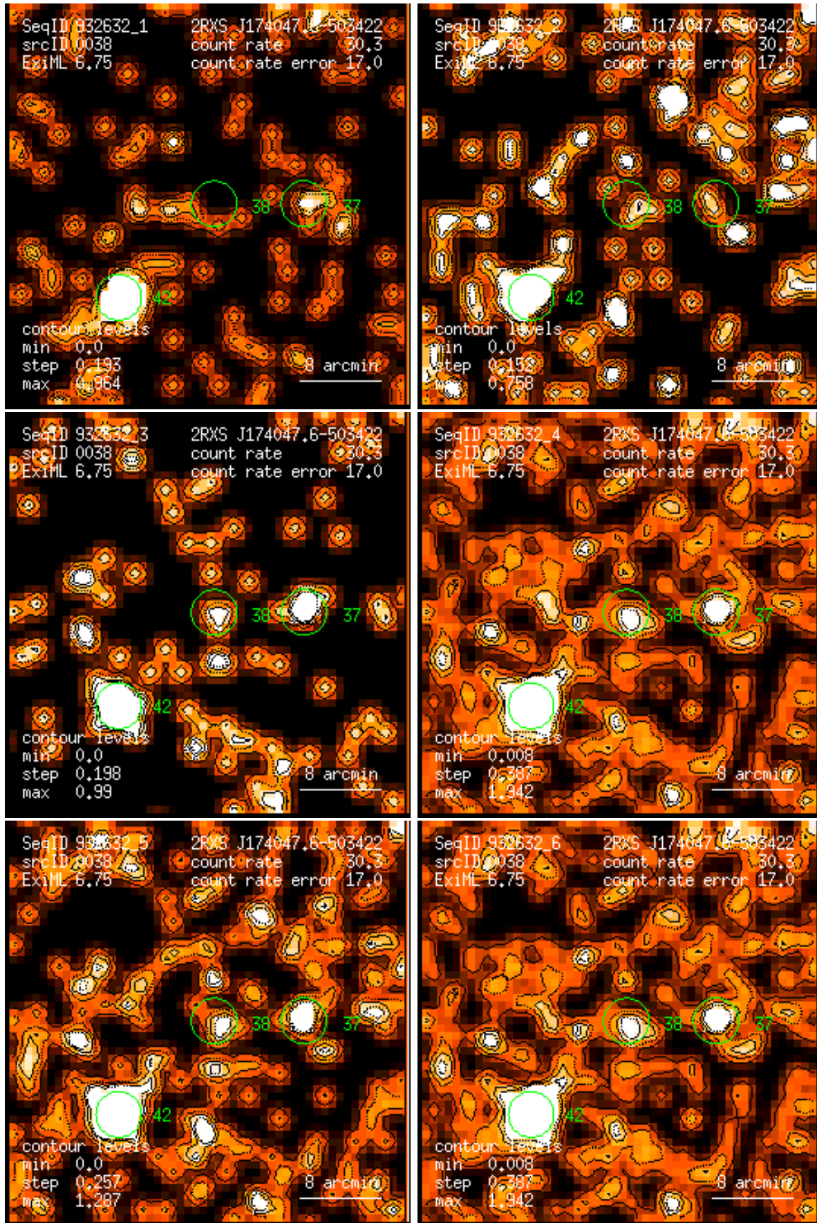
Figure 38: RASS 932632: detection 0038: band rate images, Gaussian filter: (1) PSPC channels 11 – 41, (2) 52 – 90, (3) 91 – 201, (4) 11 – 235, (5) 52 – 201, (6) 11 – 201. Broad band rates in counts/ks. Band rate contour levels in counts/ks/arcmin 2 .
