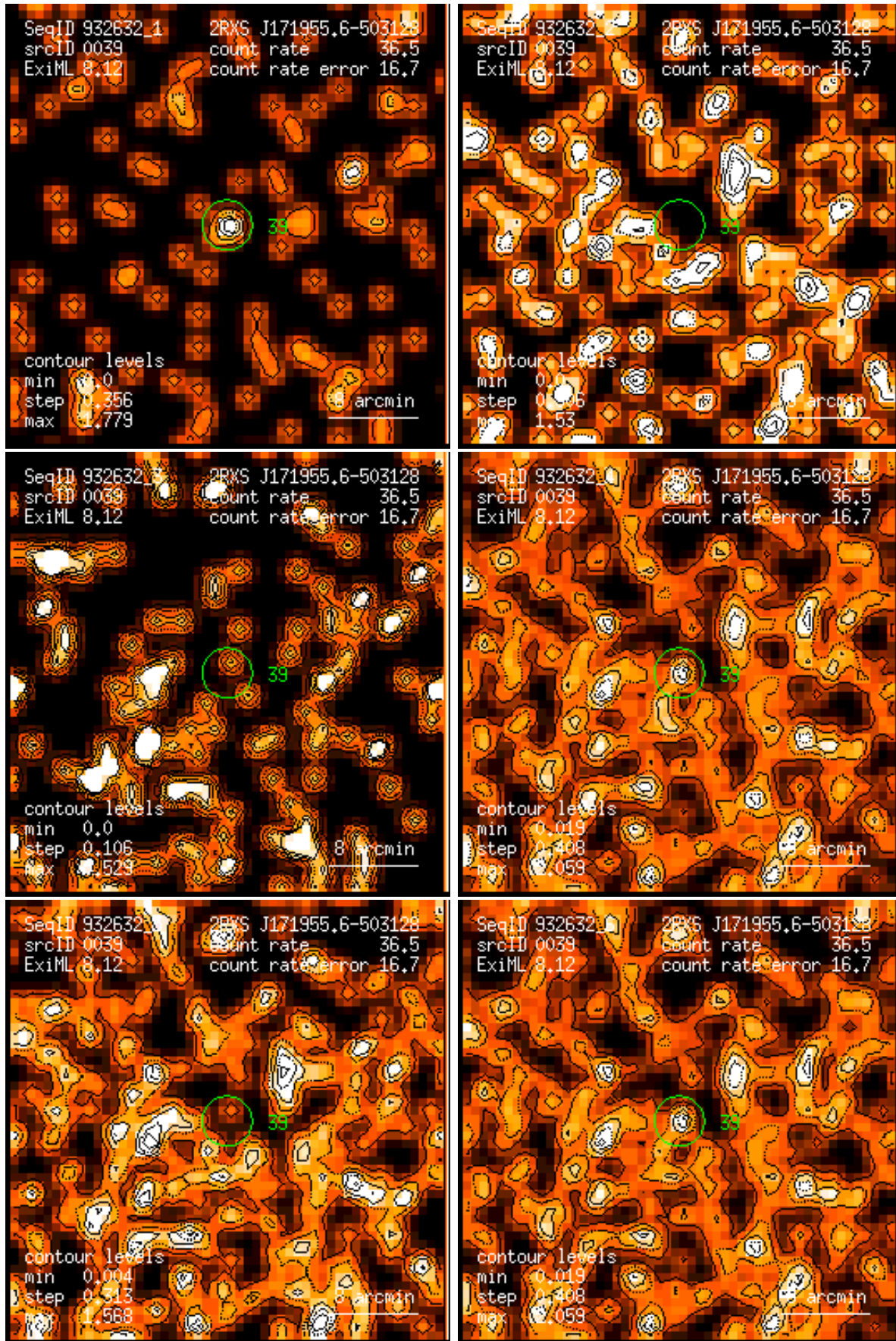
Figure 39: RASS 932632: detection 0039: band rate images, Gaussian filter: (1) PSPC channels 11 – 41, (2) 52 – 90, (3) 91 – 201, (4) 11 – 235, (5) 52 – 201, (6) 11 – 201. Broad band rates in counts/ks. Band rate contour levels in counts/ks/arcmin 2 .
