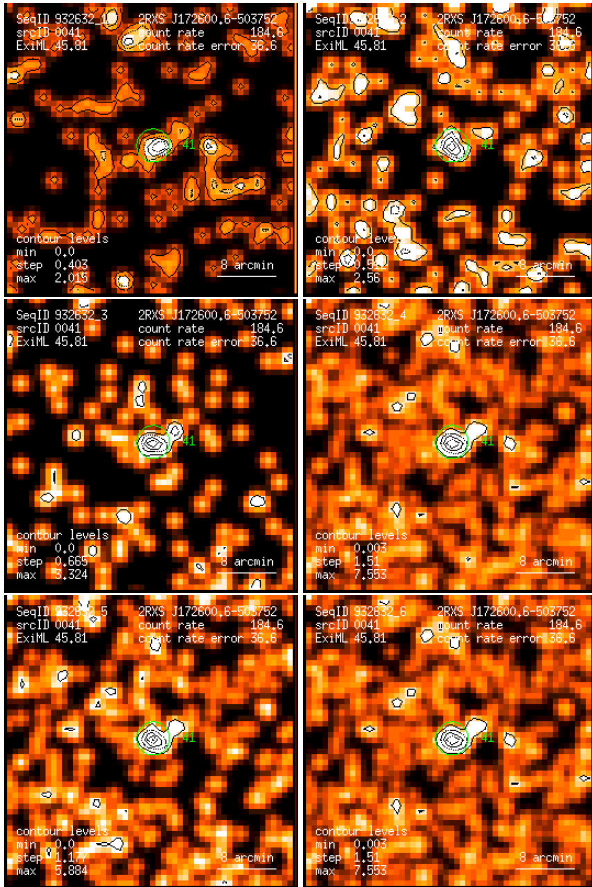
Figure 41: RASS 932632: detection 0041: band rate images, Gaussian filter: (1) PSPC channels 11 – 41, (2) 52 – 90, (3) 91 – 201, (4) 11 – 235, (5) 52 – 201, (6) 11 – 201. Broad band rates in counts/ks. Band rate contour levels in counts/ks/arcmin 2 .
